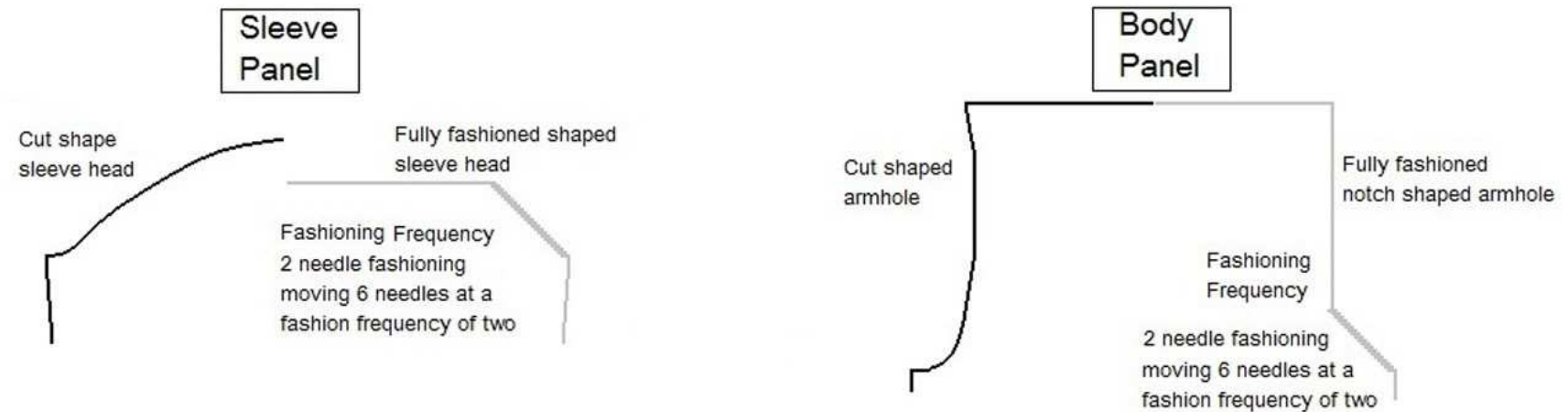
Diagram 1. Half a traditionally cut armhole shape (cut and sew), compared with that of a knitted fully-fashioned panel.
