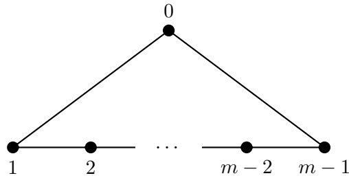
FIGURE 1. The cyclic quiver.
