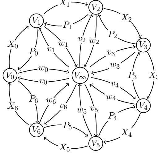
FIGURE 3. The doubled cyclic quiver for m = 7 with the modified framing.
