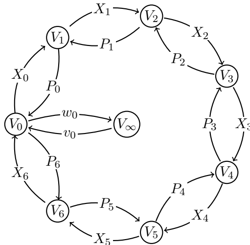
FIGURE 2. The doubled cyclic quiver for m = 7 with a special framing.
