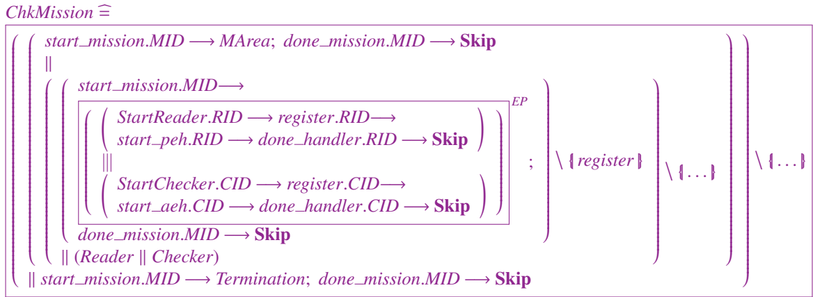
Figure 17: ChkMission after Step 1(d) of mission-sequencer-CF
