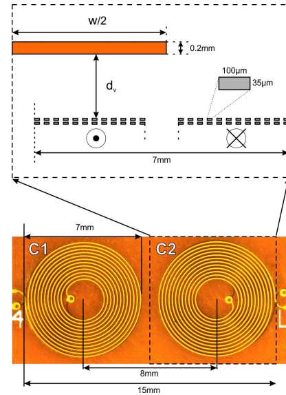
Fig. 5. Diagram of the geometry of the computational simulation. The diagram indicates a half of the simulated two coil cross-section. Each coil was represented by two 2 \times 12 arrays of wires separated by a 2.2mm gap representing the centre of the coil. Each wire section was modelled as a rectangle of dimensions 100\ \mu\text{m} \times 35\ \mu\text{m} . One half of each coil had current directed into the plane, while the opposing side current out of the plane.
