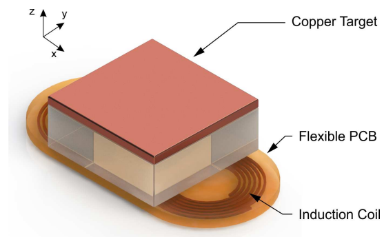
Fig. 1. A two-axis SITS. Two inductance coils are positioned below a copper target and silicone elastomer to detect forces in the z and x axes.
