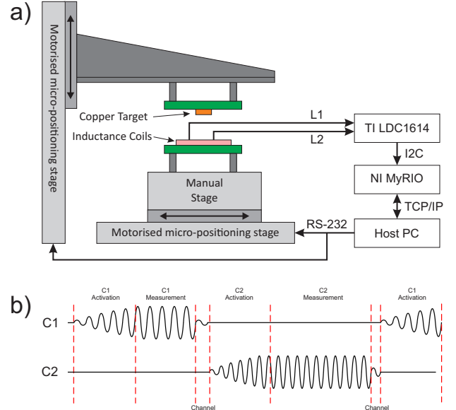
Fig. 3. a) The experimental test platform used to evaluate the 2-axis SITS and the inductive coil pair used in the system. b) Operation principle of the TI LDC1614. Each channel is operated sequentially, such that only one coil is activated at any one time.
