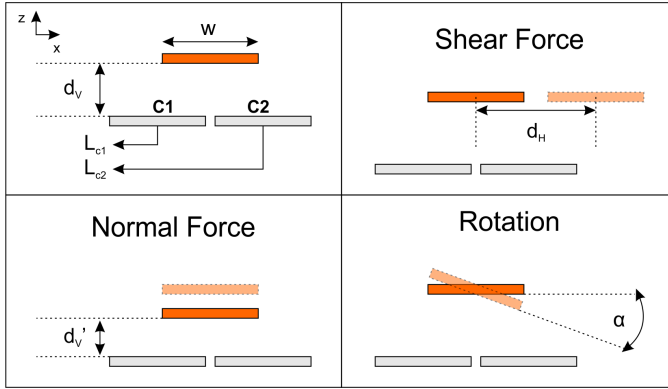
Fig. 2. Indication of the parameters of target movement in a two axis soft inductive tactile sensor (indicated in Figure 1). Parameters: d_v = vertical target displacement; d_h = horizontal target displacement; \alpha ; w = target width; C1,2 = Coil 1 & Coil 2; L_{c1,2} = Inductance C1 & C2
