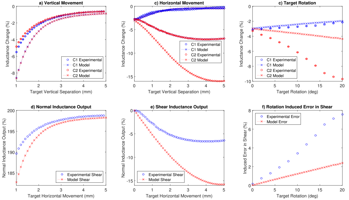
Fig. 6. Percentage change of inductance ( \Delta L/L_0 ) for a) Vertical Movement, b) Horizontal Movement, and c) target rotation. Overall outputs for d) Vertical Movement (Eq.2) and e) Horizontal Movement (Eq.1). f) The error in shear induced by the rotation.
