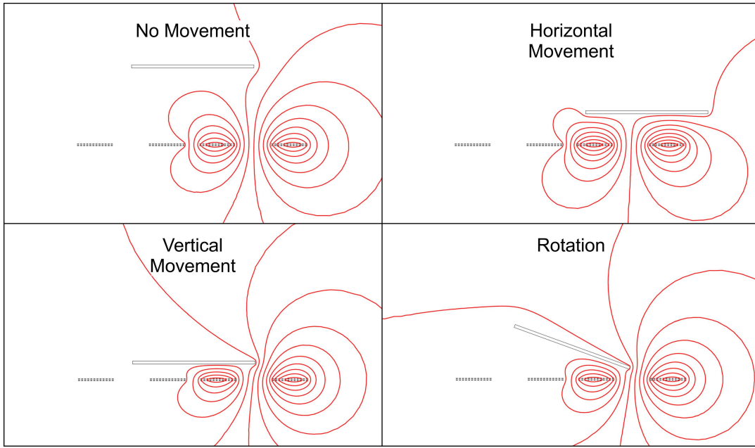
Fig. 4. The magnetic field generated by coil 2 during sequential activation under the test conditions shown in Fig.2. The magnetic field is morphed dependent on the displacement and rotation of the target. Gradient lines indicate magnetic vector potential perpendicular to the plane (Wb/m)
