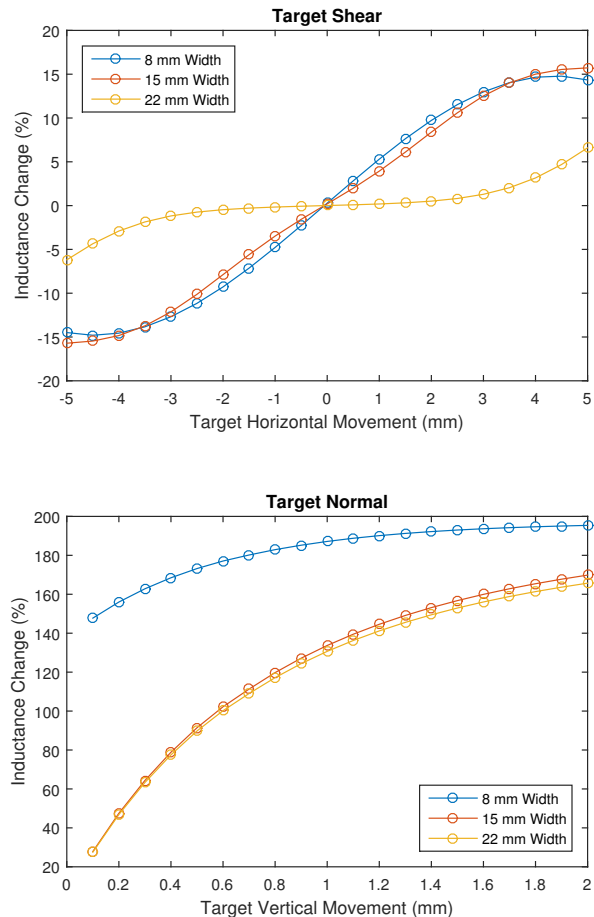
Fig. 7. Inductance change ((L_{c1} - L_{c2})/L_0) , and (L_{c1} + L_{c2})/L_0 with varying horizontal and vertical target placements
