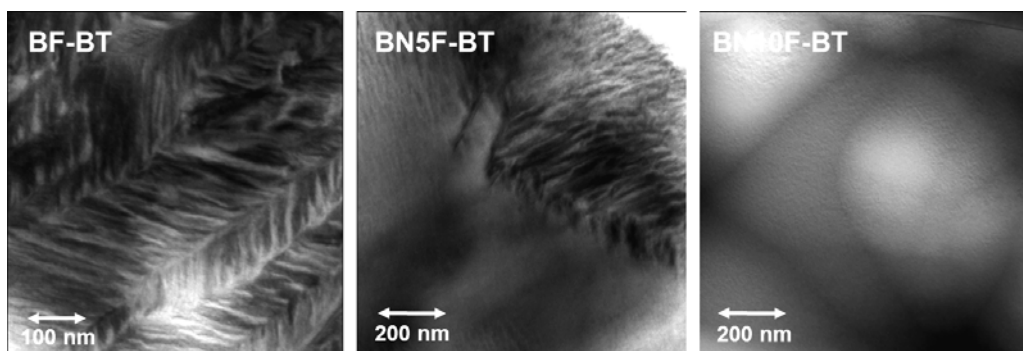
Fig. 10. TEM images of the domain structure in 0.7BF-0.3BT, 5%Nd-doped 0.7BF-0.3BT and 10%Nd-doped 0.7BF-0.3BT. 61
