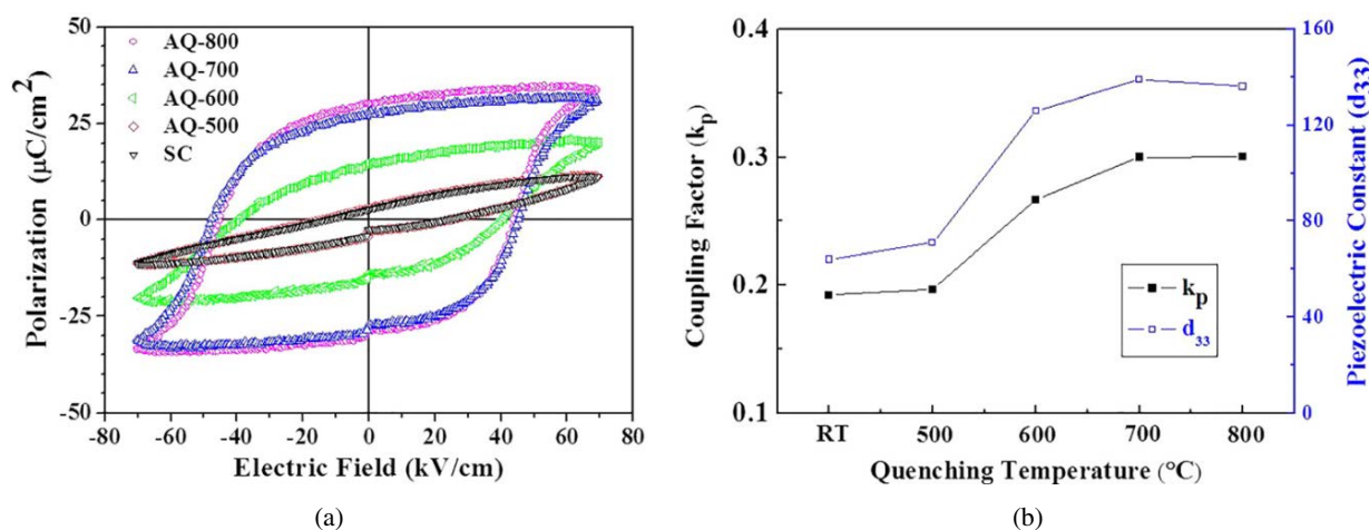
Fig. 22. (a) P - E hysteresis loops and (b) d_{33} and k_p of the slowly cooled sample (SC) and air-quenched 0.75BiFeO 3 -0.25BaTiO 3 samples from 800, 700, 600, and 500 ^{\circ}\text{C} (AQ-800, AQ-700, AQ-600, and AQ-500). 62
