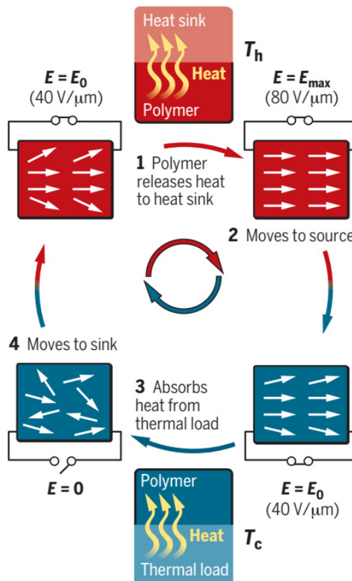
Fig. 46. Two half-cycles in Carnot cooler cycle. 221
