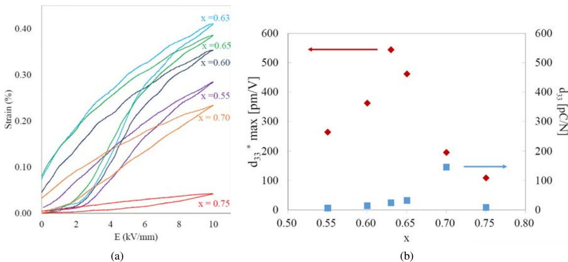
Fig. 26. (a) Unipolar S - E curves; (b) d_{33} and d_{33}^* of unpoled \text{Bi}(\text{Mg}_{2/3}\text{Nb}_{1/3})\text{O}_3 (BMN) doped BF-BT (BT- x BF-BMN, x = 0.55, 0.60, 0.63, 0.65, 0.70, \text{ and } 0.75 ) ceramics. 56
