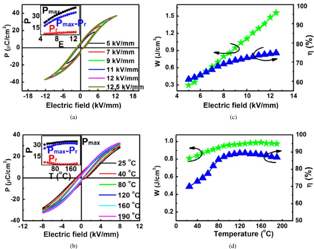
Fig. 38. P-E loops under different (a) electric fields and (b) temperature for 0.06Ba(Mg 1/3 Nb 2/3 )O 3 (BMN) doped BF-BT (BF-BT-0.06BMN) ceramic, and both W and \eta values as a function of (c) electric field and (d) temperature. 144
