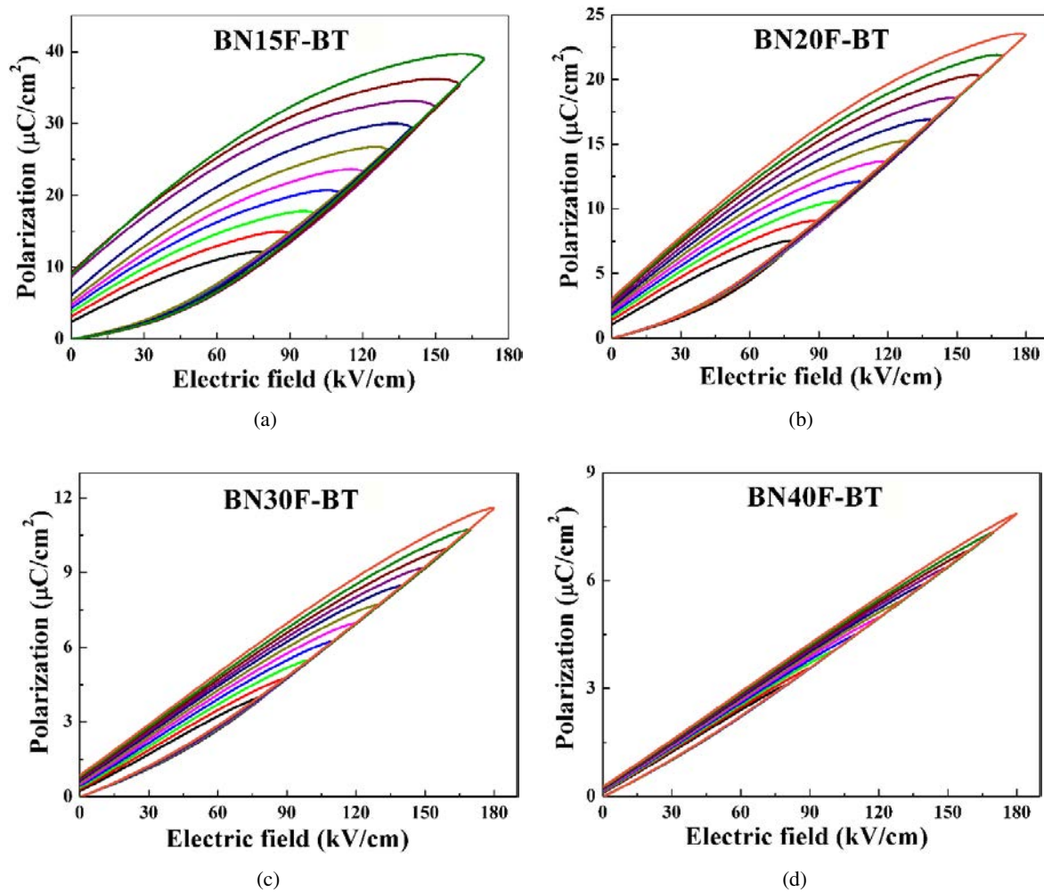
Fig. 33. Unipolar P - E loops under different electric fields for Nd doped 0.75\text{BF-}0.25\text{BT} ( \text{BN}100\text{xF-BT} ) (a) BN15F-BT, (b) BN20F-BT, (c) BN30F-BT and (d) BN40F-BT. 61
