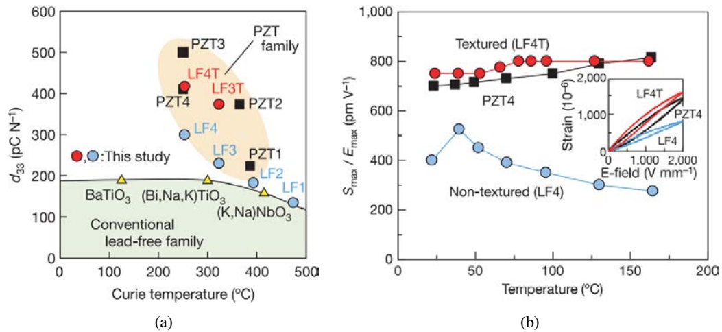
Fig. 2. (a) Comparison of d_{33} at 25^{\circ}\text{C} among developed (\text{K}_{0.44}\text{Na}_{0.52}\text{Li}_{0.04})(\text{Nb}_{0.86}\text{Ta}_{0.10}\text{Sb}_{0.04})\text{O}_3 (LF) ceramics, and conventional PZT and lead free ceramics as a function of T_c . (b) Temperature dependences of d_{33}^* for the textured (LF4T), nontextured (LF4) and PZT4 ceramics. Inset, electric-field-induced strain curve for LF4T, LF4 and PZT4 ceramics at 25^{\circ}\text{C} . 16
