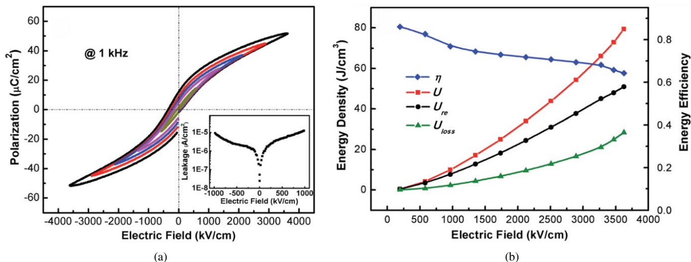
Fig. 45. (a) P - E loops of 0.4BiFeO 3 -0.6SrTiO 3 (BF-ST) film with various applied electric fields at 1 kHz. The inset is the J of BF-ST film at various DC biased electric fields. (b) Stored energy density U , recoverable energy density U_{re} , hysteresis loss U_{loss} , and \eta as a function of the applied electric field. 220
