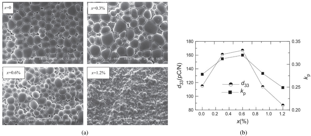
Fig. 18. (a) SEM images and (b) d_{33} and planar electromechanical coupling factor k_p of 0.71\text{BiFe}_{1-x}\text{Co}_x\text{O}_3-0.29\text{BaTiO}_3 + 0.6\text{ wt\% MnO}_2 (BFC x -BT) ceramics. 87
