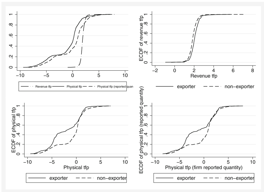
Fig. 4 Productivity distribution
