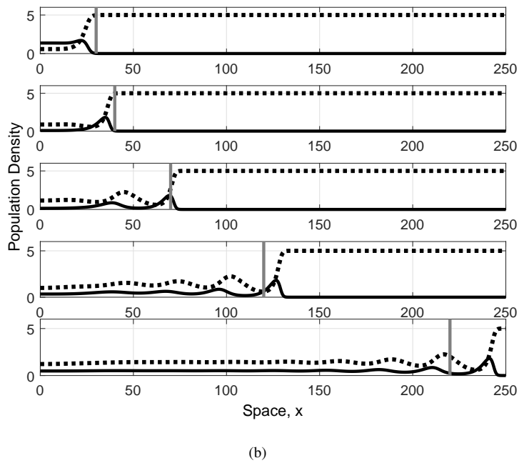
Fig. 2 Predator invasion in the absence of disease. Attractive preytaxis. (a) shows the initial stages of predator invasion, where the predators grow locally up to steady state and spread to converge to the shape of the travelling wave. (b) shows that after this convergence, the wave travels faster than the analytic speed. The times and lines used are the same as in Figure 1. Parameter values: Same as in Figure 1, except F_S = 1 .
