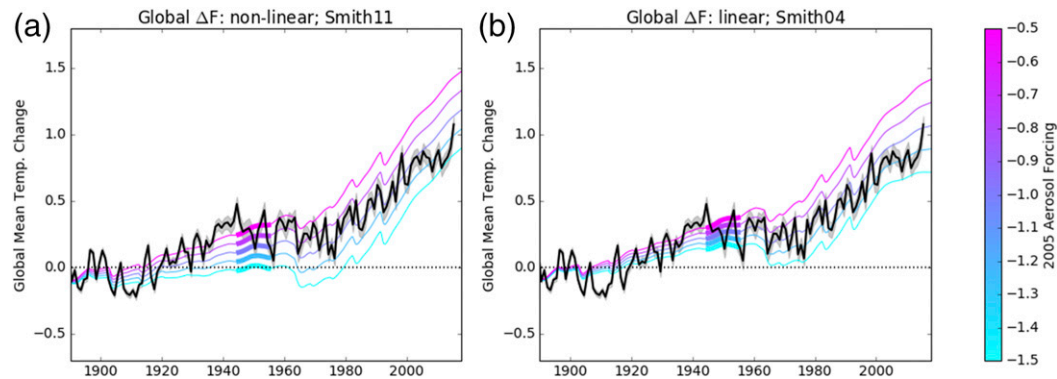
FIG. 2. (a) The time series illustrating the dependence of global mean temperatures when varying on the magnitude of global 2005 aerosol forcing (denoted by the color bar) from an energy balance model/simple climate model [described in Harris et al. (2013)]. The temperatures in the 11 years centered around 1950 are highlighted by the thicker lines. The \text{SO}_2 emissions are taken from Smith et al. (2011) and the indirect component of the global forcing is treated as logarithmic to these emissions (as per S15). The other simple model parameters are set at “central” values (climate sensitivity = 3 K; 2 \times \text{CO}_2 radiative forcing = 3.71 \text{ W m}^{-2} ; land–sea contrast = 1.4; fraction of aerosol forcing treated as linear = 0.22; background natural emissions = 31.3). The mean (black) and uncertainty range (gray) for an observational estimate of historical temperature change from Morice et al. (2012) are shown for comparison. (b) As in (a), but using Smith et al. (2004) \text{SO}_2 emissions and treating the global forcing as a linear function of these emissions.
