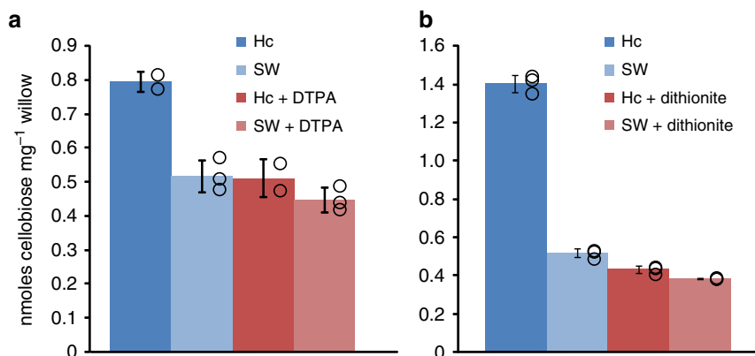
Fig. 5 Digestibility of willow following short hemocyanin pretreatments at room temperature. Digestibility of willow measured as release of cellobiose (nmol) per unit biomass (mg) in saccharification reactions upon biomass pretreatment. Pretreatment of willow with hemocyanin in seawater (Hc, dark tones) or seawater alone (SW, light tones) without (blue colors) and with (+, red colors) 50 mM DTPA (chelator) for 10 min ( a ) or 50 mM dithionite (reducing agent) for 20 min ( b ), followed by saccharification with CBH I from Hypocrea jecorina (HjCBH I). Hydrolysates were analyzed by HPAEC against cello-oligomer standards, and values normalized to reactions without CBH following pretreatments to account for any remaining cellulase activity derived from the hemocyanin preparation. Circles represent sample values and bars sample mean \pm SD, N = 3 ( N = 2 for Hc \pm DTPA)
