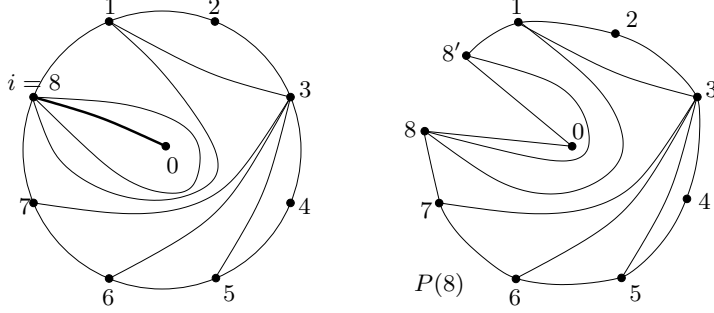
FIGURE 10. Type (iv), i = 8 .
