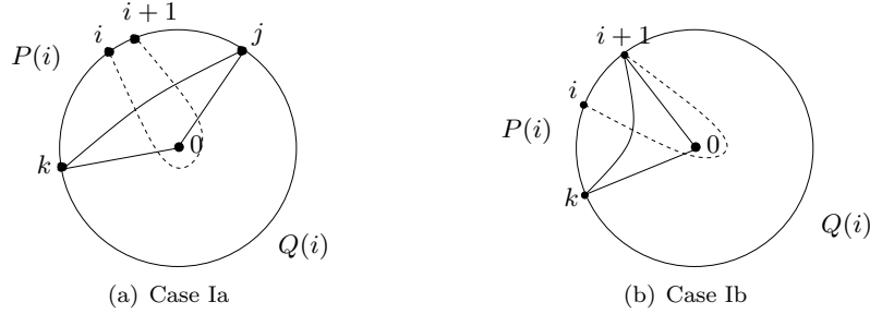
FIGURE 21. Proof of Proposition 5.8(3), Cases (Ia) and (Ib).
