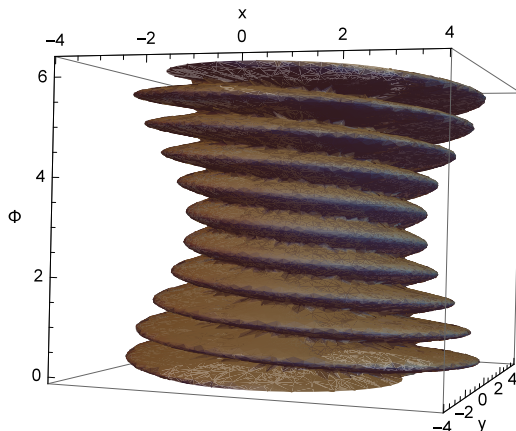
FIG. 1. Outer separatrix sheet Z = A as a function of x , y and \Phi , m = 2 , \epsilon = 10^{-1} , \varpi = 1 , r_c = 2 , \tau_3 = 0 , and A(\Phi) = [1 + \cos(\Phi)/2]^2 .
