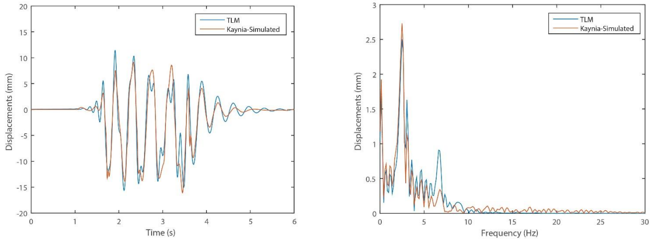
Figure 11: Track displacement for Southbound train at 200 km/h (case 3) in time domain (Left) and frequency domain (Right)
