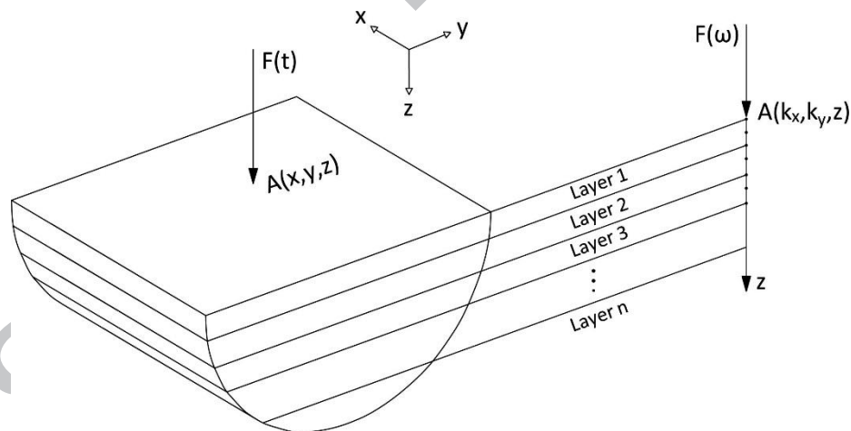
Figure 3: Schematic drawing of the procedure of the vertical discretization and domain transform in the thin-layer method
