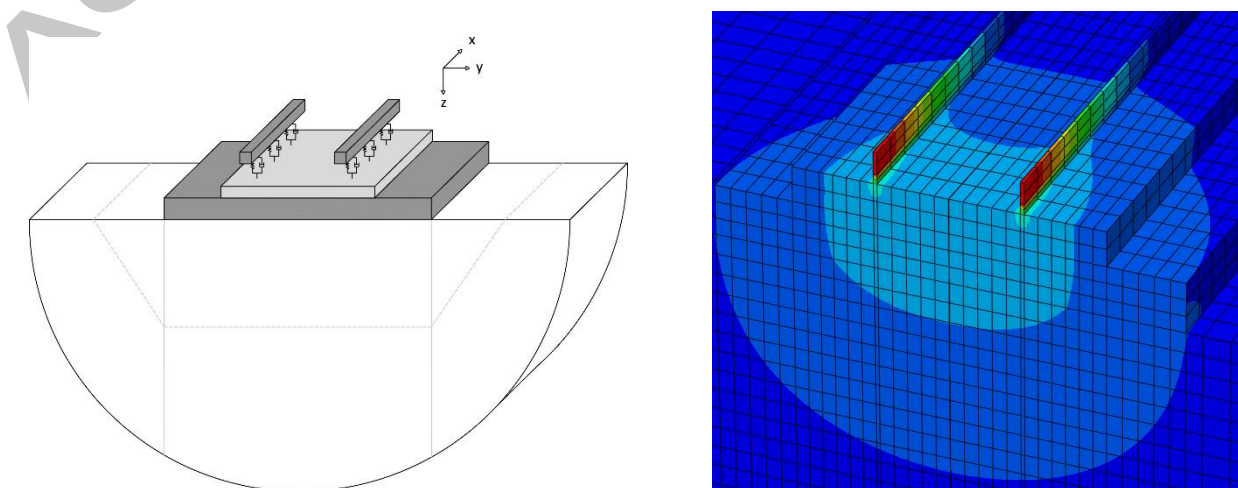
Figure 5: Left: Layout of soil replacement geometry, Right: Cut through ABAQUS model showing track and soil response during receptance test
