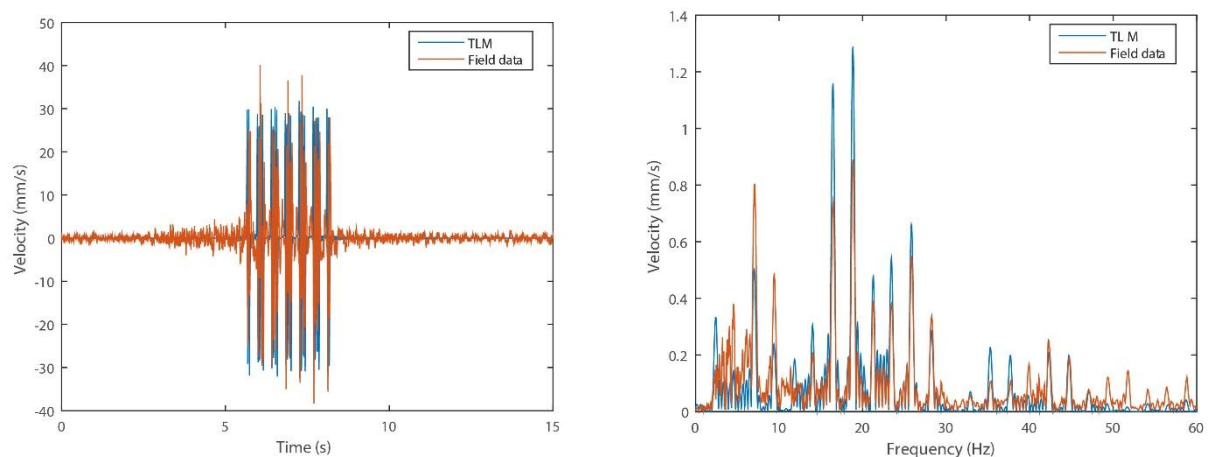
Figure 14: Vertical sleeper velocity due to the train passage in both time content (Left) and in frequency content (Right)
