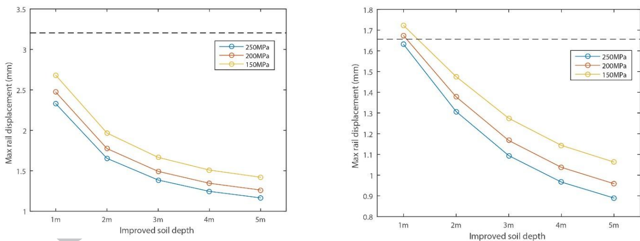
Figure 15: Maximum vertical rail displacement for Soil 1. (Left) Ballasted track; (Right) Slab track; Dashed black line represents the original value
