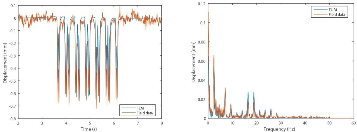
Figure 13: Rail displacement due to the train passage in both time content (Left) and in frequency content (Right)
