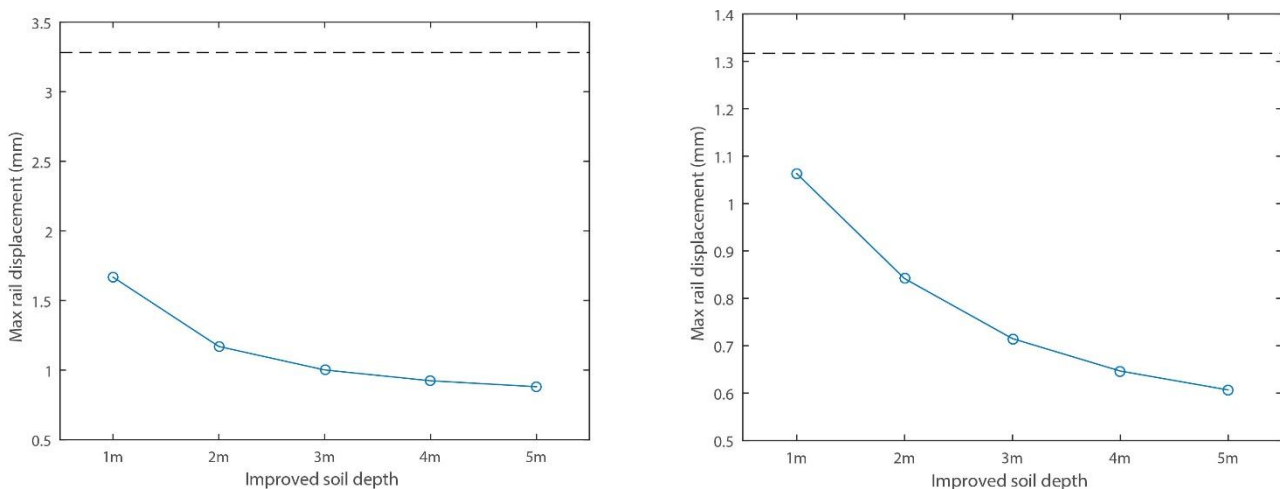
Figure 18: Maximum vertical rail displacement for Soil 2. (Left) Ballasted track; (Right) Slab track; Dashed black line represents the original value
