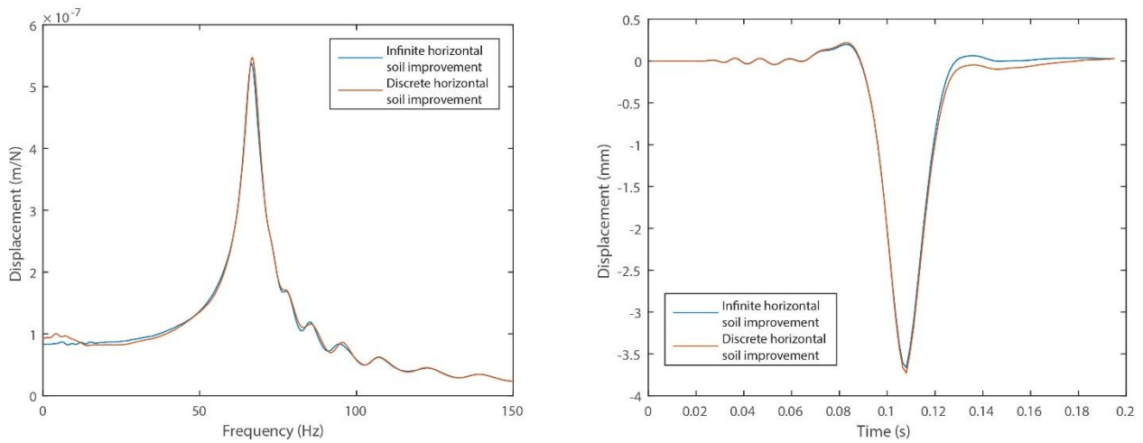
Figure 6: Comparison between simplified and detailed soil replacement geometry (Left: static rail receptance excitation, Right: moving load excitation time history)
