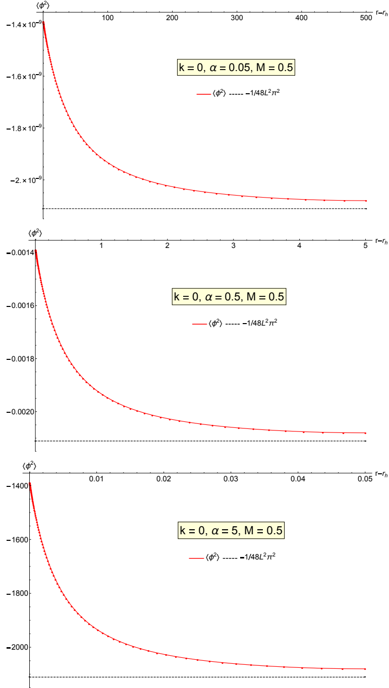
Figure 4. Renormalized VP (red curves) for a massless, conformally-coupled scalar field on an asymptotically adS black hole with k = 0 , mass M = 0.5 and three values of the space-time parameter \alpha : \alpha = 0.05 (top), \alpha = 0.5 (middle) and \alpha = 5 (bottom). The results for \alpha = 0.05 and \alpha = 5 are obtained from those for \alpha = 0.5 by applying the scaling (5.10). This scaling leaves the dimensionless radial coordinate \zeta unchanged and thus the renormalized VP is shown as a function of the dimensionful radial coordinate r . The black dotted lines denote the renormalized VP for a massless, conformally-coupled scalar field in pure adS space-time (5.6).
