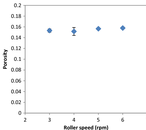
Fig. 8 The porosity of ribbon produced at different roller speed
