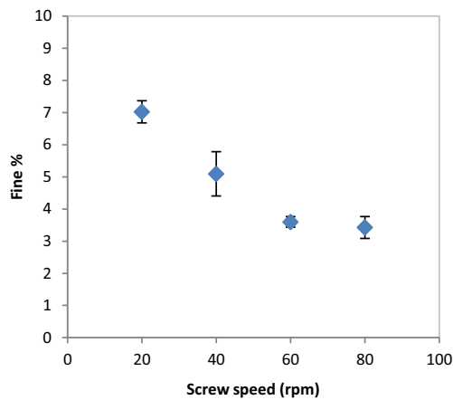
Fig. 19 Percentage of fines produced at different feeder screw speed
