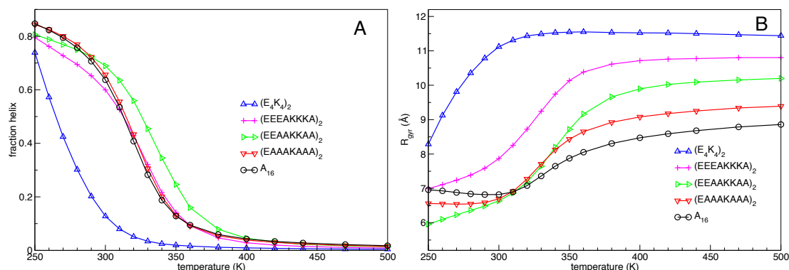
Figure 5. Helicity (A) and radius of gyration (B) of peptides where, starting from (E_4K_4)_2 , alanines are introduced preserving the 4-4 pattern of charged residues. The peptide with the pattern EEAAKKAA appears to have the highest melting temperature.
