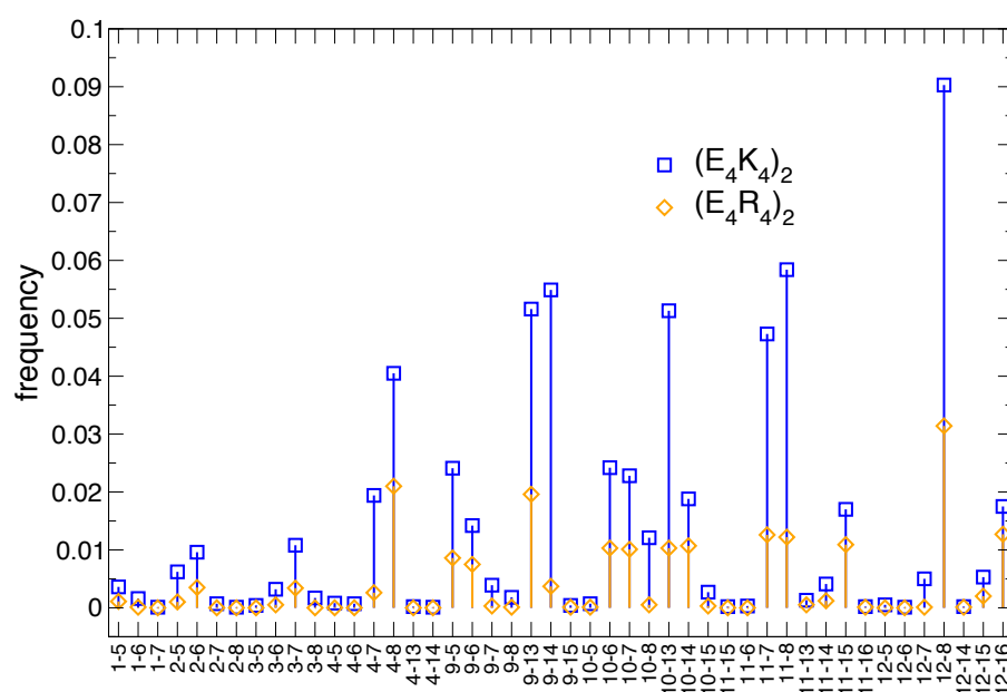
Figure 6. Frequency of salt bridges at 250 K for two polyampholyte helical sequences. Salt bridges are more frequent for (E_4K_4)_2 than for (E_4R_4)_2 despite the latter having larger helical content. Strength of salt bridges does not appear to correlate with helicity. Residues numbered 1-4 and 9-12 are E, those numbered 5-8 and 13-16 are K or R.
