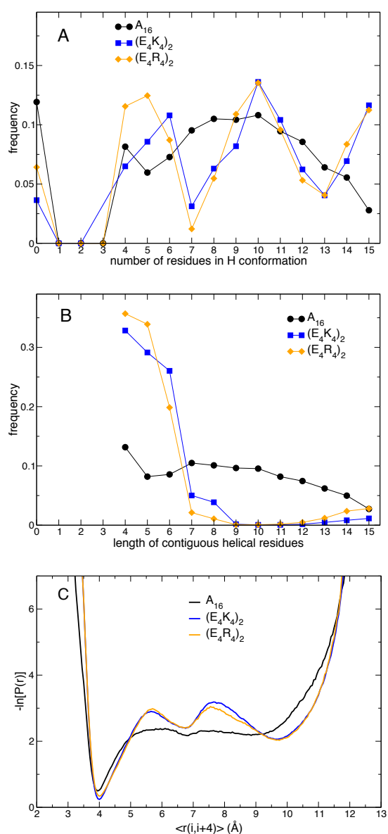
Figure 4. Different nature of helices. (A) Frequency of conformations with a given number of residues in a helical conformation at the lowest temperature (250 K). For A_{16} the maximum frequency is \sim 10 but any number is similarly likely between the minimum (4) and the maximum (15). For the two helical polyampholytes we observe an intriguing pattern where residues in helical conformations seem to occur most likely in multiples of \sim 5 . (B) Frequencies of occurrence of contiguous stretches of residues in helical conformation. This is again relatively smooth for A_{16} . For polyampholyte helical peptides the length of helices is mostly 4–6 amino acids, which suggests helices do not propagate beyond that length or merge but exist independently. (C) Negative logarithm of the probability of the helix hydrogen bond distance. This is the distance between the amide nitrogen of an amino acid and the carbonyl carbon of the amino acid four residues earlier, averaged over all possible pairs of residues. Profiles are shown for temperatures at which peptides are \sim 40\% helical.
