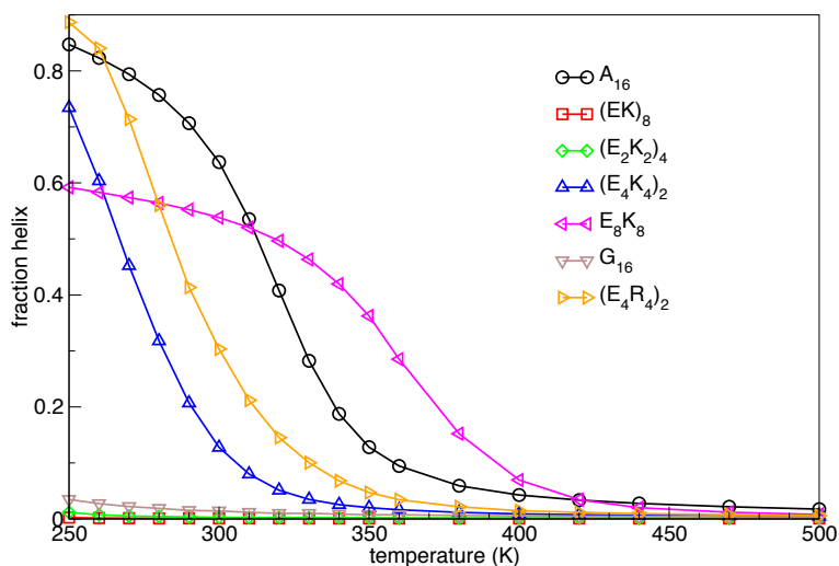
Figure 1. Helicity. At the lowest temperature A_{16} , (E_4K_4)_2 and (E_4R_4)_2 are highly helical. Polyampholyte sequences lose helicity faster with increasing temperature, and (E_4R_4)_2 is at all temperatures more helical than (E_4K_4)_2 . E_8K_8 is mostly helical in its C-terminal part and loses helicity only at high temperature.
