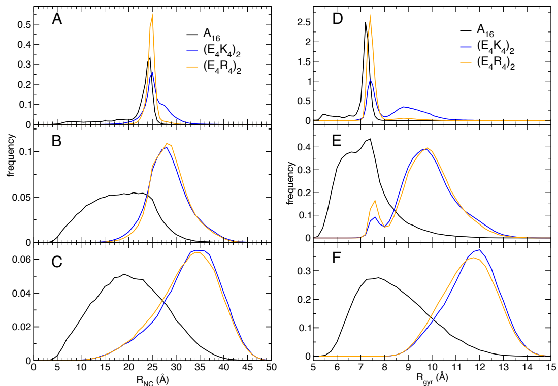
Figure 3. Histograms of r_{NC} (left) and R_{gyr} (right). (A,D) At the lowest temperature (250 K). (B,E) At a temperature in which all peptides are ~40% helical. (C,F) At 380 K when all peptide are <5% helical.
