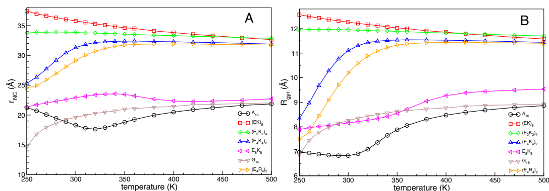
Figure 2. (A) Average end-to-end distance and (B) radius of gyration at a function of temperature. At the lowest temperature, all sequences with helical propensity are extended with a length around 24 Å (length of a perfect 16 amino acid helix). A_{16} gets shorter when it loses helicity (hydrophobic collapse) before expanding at high temperature. Helical polyampholyte sequences ( (E_4K_4)_2 and (E_4R_4)_2 ) elongate as they lose helicity.
