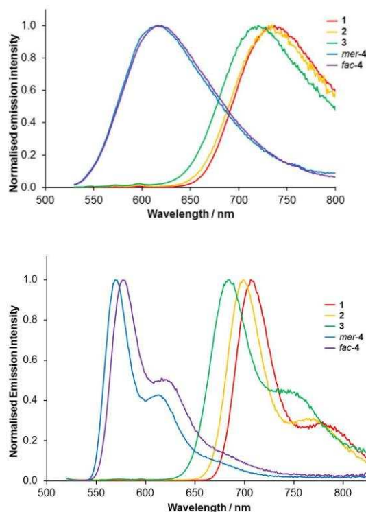
Figure 5. Top: Normalised emission spectra recorded for aerated MeCN solutions of 1-3 , mer- 4 and fac- 4 at r.t. Bottom: Low temperature emission spectra (77 K) for complexes 1-3 , mer- 4 and fac- 4 in a 4:1 EtOH:MeOH glass.
