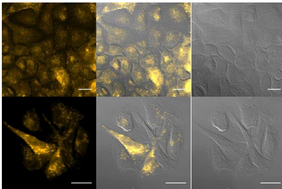
Figure 9. Confocal microscopy images of EJ bladder carcinoma cells incubated with complex 4 (20 \mu M, 6 hour incubation). Each panel comprises emission image (left, \lambda_{\text{exc}} = 543 nm, \lambda_{\text{em}} = 565\text{-}615 nm), bright-field image (right) and overlay of emission and bright-field images (centre). Scale bars = 20 \mu m.
