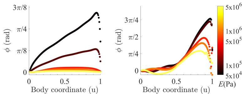
FIG. 4: Neuromechanical phase lag along the body, simulated in agar, over the same range of Young’s modulus shown in Fig. 2. Left: Under feed-forward control, lag is negligible for E \gtrsim 5 \times 10^5 Pa but increases approximately linearly for lower E . Note that for a constant undulation period T_f the phase lag \phi and time lag \Delta are related by \phi = 2\pi T_f / \Delta . Right: Under proprioceptive control, the lag is negligible in anterior half of the body and increases dramatically towards the tail ( u = 1 ).
