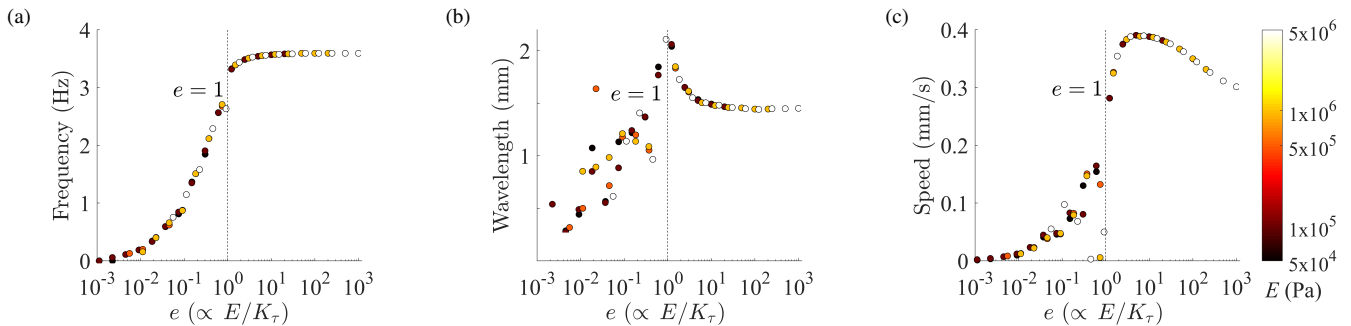
FIG. 2: The effect of environmental drag on (a) undulation frequency, (b) wavelength, and (c) the speed of the nematode in Newtonian environments ( K = 1.5 ). Simulation results spanning E - K_\tau space are plotted against the nondimensional parameter e . Outliers represent simulations exhibiting uncoordinated locomotion.
