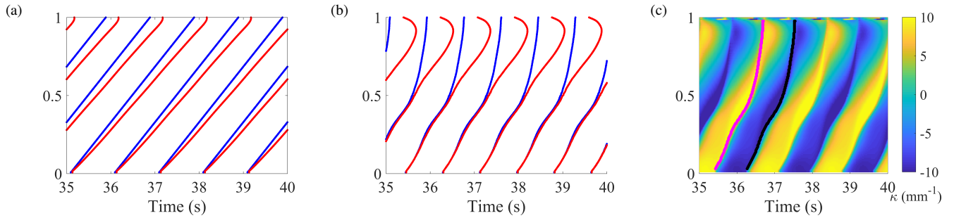
FIG. 5: Zero contours of the muscle torque, \beta(u, t) (blue) and body curvatures, \kappa(u, t) (red), obtained from simulations in an agar-like medium and E = 100 kPa. (Both positive and negative crossings are included.) (a) Under a model of feed-forward (CPG) control, the latency between activation and body bend grows linearly along the body. (b) Under a model of proprioceptive control with a diminishing proprioceptive range in the posterior half of the body, the curvature and muscle activation are tightly coupled in the anterior half; the increasing phase lag towards the tail arises from an accelerated neuromuscular wave speed of muscle torque in the posterior half of the body. (c) Kymograms of the body curvature corresponding to (b). Black and magenta lines show peak negative and positive values of muscle activation \beta(u, t) along the body, respectively.
