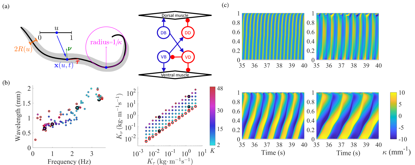
FIG. 1: A continuum neuromechanical model reproduces the swim-crawl transition. (a) Model schematic describing geometry (left) and neural circuit (right). (b) Frequency-wavelength relationship (left) plotted for a wide set of drag coefficients, K = K_v/K_t (right), including Newtonian environments (red circles). Parameters used for sample kymograms (black circles) span the swim-crawl transition. (c) Curvature kymograms (showing the curvature along the body along the vertical axis from head, at u = 0 , to tail, u = 1 , and in time) in environments from water (top left) through intermediate fluids (top right to bottom left) to agar (bottom right).
