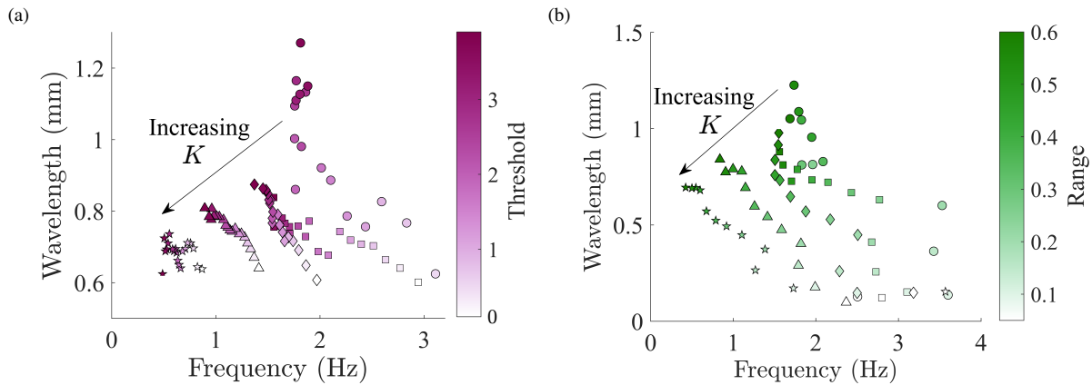
FIG. 3: Internal modulation of proprioceptive pathways gives rise to an inverse frequency-wavelength relationship. Internal neural modulation of (a) proprioceptive threshold and (b) proprioceptive range, for K = 7.5 (circles), K = 12 (squares), K = 18 (diamonds), K = 30 (triangles) and K = 45 (stars), with E = 100 kPa.
