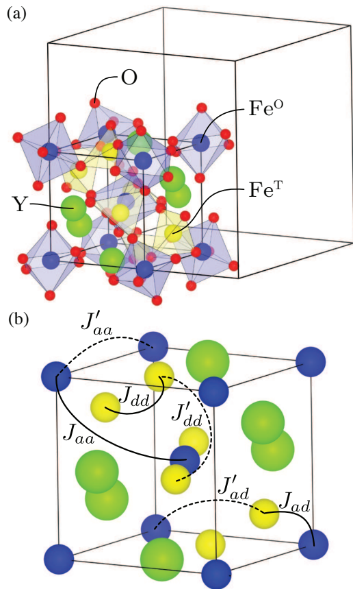
FIG. 1. (a) 1/8 of the YIG unit cell. The dodecahedrally coordinated Y ions (green) occupy the 24c Wyckoff sites, the octahedrally coordinated Fe O ions (blue) occupy the 16a sites, and the tetrahedrally coordinated Fe T ions (yellow) occupy the 24d sites. The oxygen (red) 96h sites are not confined by symmetry, while all cation sites are on special crystallographic positions. (b) The solid and dash lines denote the nearest and next nearest neighbor exchange interactions. The subscripts aa , dd and ad stand for the Fe O -Fe O , Fe T -Fe T and Fe O -Fe T interactions, respectively.
