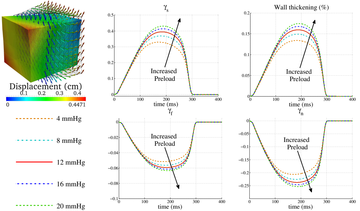
Figure 6: Test 2: The transmurial cube is preloaded with an endocardial diastolic pressure which elongates the fibers. The direct introduction of the force-length relationship (19) in (27) leads to an increase wall thickening when the preload is increased. Top left: initial configuration (grid), fiber field (arrows) for 16 mmHg of preload and wall thickening at maximum contraction. The displacement magnitude is computed with respect to the preloaded configuration. Top center and top right: macroscopic active strain in sheetlet direction \gamma_s and wall thickening for different values of initial preload. Bottom center and bottom right: macroscopic fiber and cross-fiber strains \gamma_f and \gamma_n for different values of initial preload.
