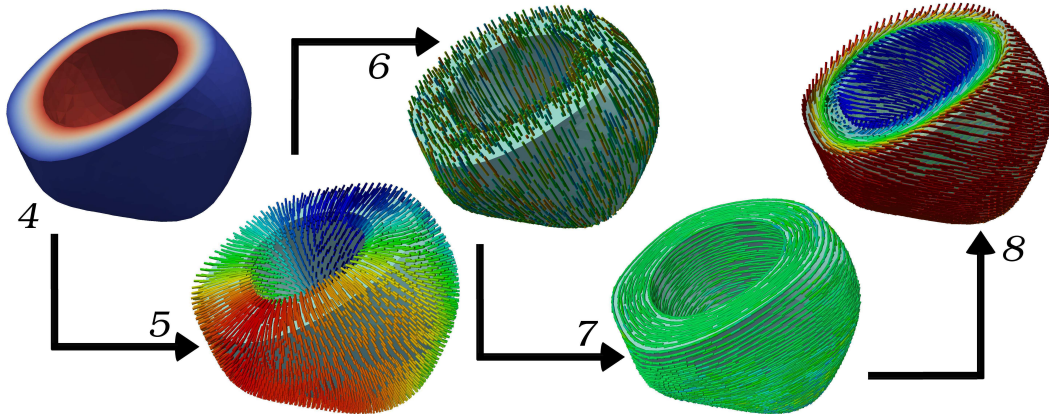
Figure 4: Steps to create the sheetlets and fiber directions. Referring to steps 4 - 8 in Algorithm 1, following the arrows: step 4) solution of problem (23); step 5) sheetlet direction \mathbf{s}_0 ; step 6) projection vector \mathbf{k}_p/\|\mathbf{k}_p\| ; step 7) flat fiber field \tilde{\mathbf{f}}_0 ; step 8) fiber field \mathbf{f}_0 .
