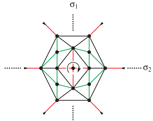
Fig. 8. A Schlegel-like diagram of a triangulated spherical polyhedron which yields the Sarrus linkage in Fig. 9(a) if the central vertex and the vertex ‘at infinity’ together with their incident edges (shown in red) are removed, and each vertex to four green edges is duplicated and coned over the same neighbours. Both the underlying polyhedron and the Sarrus linkage have maximum symmetry C_{2v} , as indicated. Note that swapping the roles of green and red edges yields the Stewart platform in Fig. 10. (For interpretation of the references to colour in this figure legend, the reader is referred to the web version of this article.)
