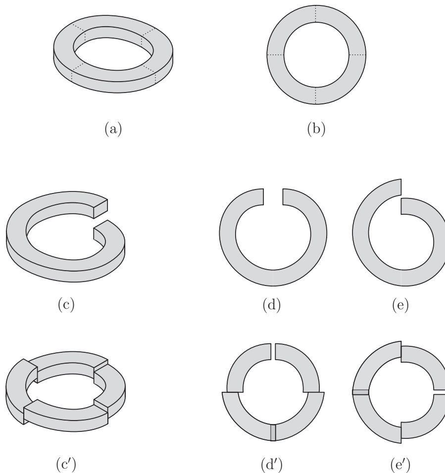
Fig. 3. A depiction of the extra local states of self-stress in a panel-hinge block-and-hole polyhedron. At a vertex, edges and panels come together so that a continuous ring of material is formed, although of infinitesimal extent. This ring is shown in isometric view in (a), and along a radius of the underlying object in (b): four potential ‘cut’ lines are shown. An independent set of three states of self-stress is here visualized by considering the shape the ring would take up if cut to relieve the internal stresses. In (c)–(e) the ring is cut in just one place, while in (c′)–(e′) the ring is cut in four places; it is clear from this that (d′) and (e′) form a pair, with one state of self-stress just the rotated version of the other. These states of self-stress are intrinsic: they cannot be relieved by bending around the hinges intersecting at the vertex.
