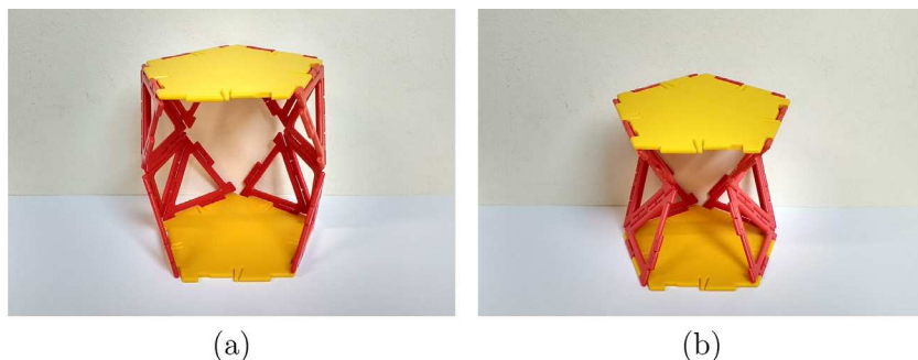
Fig. 11. A Polydron model of a finitely flexible panel-hinge structure with point group C_{2v} (a), and a point on the path of the mechanism (b).
