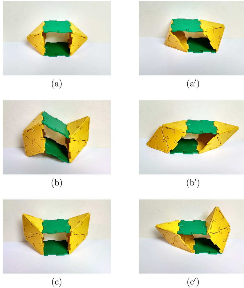
Fig. 12. Polyhedron models of finitely flexible symmetric block-and-hole structures that are strongly counting-balanced. For the structures in (a), (b) and (c), figures (a'), (b') and (c') show a point on the path of the corresponding mechanism.
