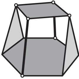
Fig. 10. A Stewart platform obtained by swapping blocks and holes in the Sarrus linkage shown in Fig. 9(a). Open circles indicate pin joints; there are two hinge joints connecting hexagonal and triangular panels.
