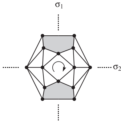
Fig. 5. A counting-balanced, but not strongly counting-balanced, block-and-hole framework with two pentagonal blocks and two holes with perimeters 4 and 6, respectively. The Schlegel diagram for the panel-hinge version shows the maximum possible C_{2v} symmetry, indicating the presence of a two-fold rotation and two perpendicular mirror planes.
