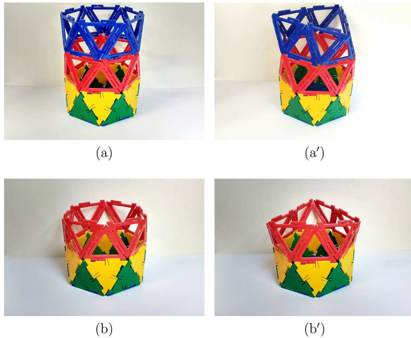
Fig. 13. (a),(b) Polydron models of flexible tower structures with a hexagonal block and hole; (a'), (b') points on the paths of the corresponding mechanisms.
