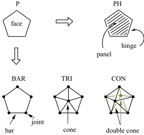
Fig. 2. A set of objects related to the polyhedron \mathcal{P} : a panel-hinge model of \mathcal{P} (PH); a bar-joint model of the polyhedron (BAR); a fully triangulated bar-joint polyhedron (TRI); a double-cone construction of a bar-joint model with blocks for all faces (CON).
