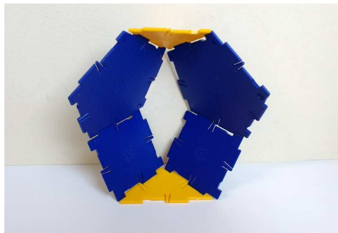
Fig. 6. A Polydron model of a block-and-hole structure of C_s (single reflection) symmetry for which the bar-joint representation is counting-balanced and symmetry-isostatic.
