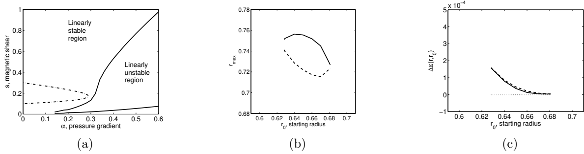
Figure 9: Plot of: (a) trajectory (dashed-dotted line) of the profile in ‘ s - \alpha ’ space; (b) plot of the location of the maximum r_{max} = r_{eq}(0, r_0) of the displaced states (the upper solid line is the \mathcal{E} = \mathcal{E}_2 state and the lower dashed line is the \mathcal{E} = \mathcal{E}_1 state) against starting flux surface r_0 ; (c) the energy change of the displaced states versus the initial position (again solid line is \mathcal{E} = \mathcal{E}_2 and the dashed line is \mathcal{E} = \mathcal{E}_1 ). Here the trajectory is further still from the linear ballooning boundary. There is no region where the displaced states have lower energy – i.e. all field lines from r_0 = 0.62 to r_0 = 0.68 are in the second category.
