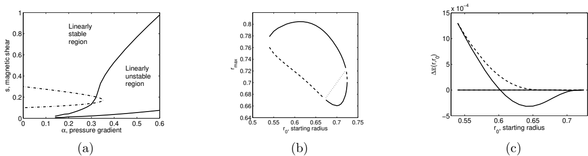
Figure 10: Plot of: (a) trajectory (dashed-dotted line) of the profile in ‘ s - \alpha ’ space. The trajectory crosses the linear ballooning boundary and therefore part of the plasma is linearly unstable. (b) plot of the location of the maximum r_{max} = r_{eq}(0, r_0) of the displaced states (the lower line is the \mathcal{E} = \mathcal{E}_2 state and the upper line is the \mathcal{E} = \mathcal{E}_1 state) against starting flux surface r_0 . The dotted line shows r_{max} = r_0 . Field lines are in the second category from r_0 = 0.54 to r_0 = 0.63 and the third category from r_0 = 0.63 to r_0 = 0.67 . From r_0 = 0.67 to r_0 = 0.72 the unperturbed state is linearly unstable (the fourth category) and one displaced state has r_{max} > r_0 and the other displaced state has r_{max} < r_0 ; (c) the energy change of the displaced states versus the initial position (lower line is \mathcal{E} = \mathcal{E}_2 and the upper line is \mathcal{E} = \mathcal{E}_1 ). From r_0 = 0.67 to r_0 = 0.72 both displaced states have negative energy 0 > \mathcal{E}_1, \mathcal{E}_2 – this is shown by making both lines solid. From r_0 = 0.72 to r_0 = 0.723 both displacements are inward and field lines are in the third category. From r_0 = 0.723 to r_0 = 0.724 field lines are in the second category.
