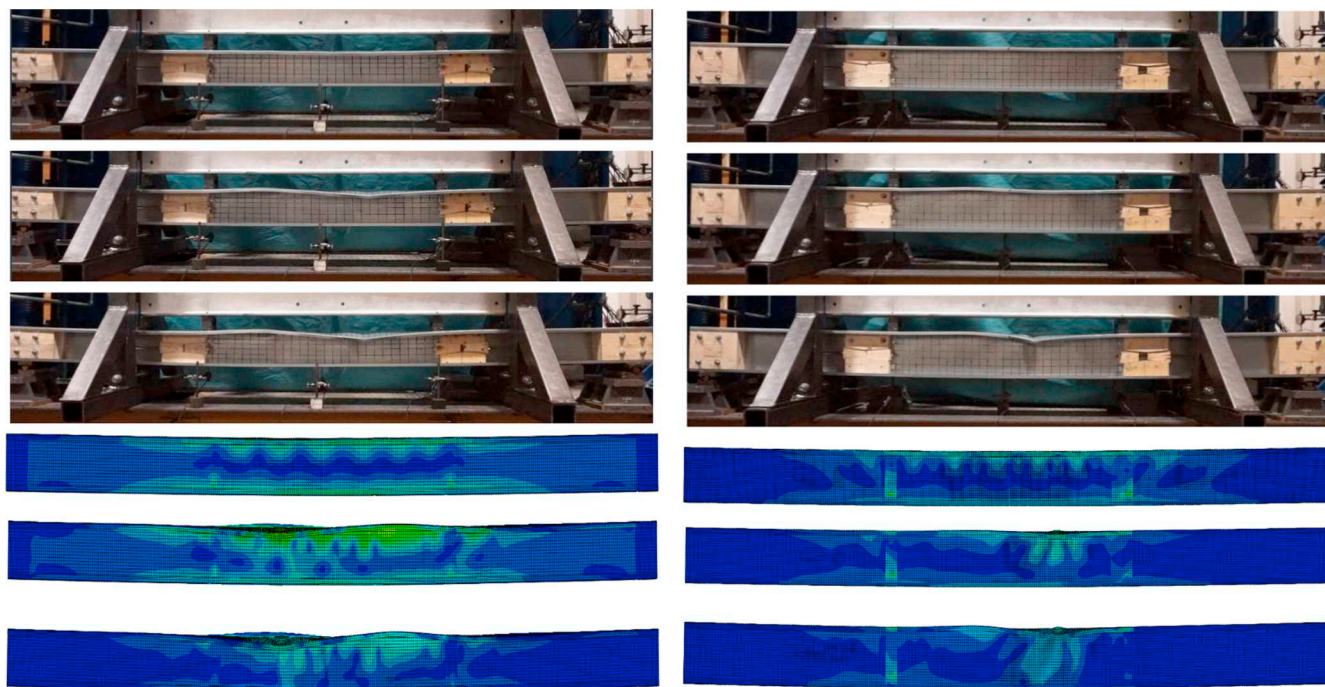
(a) Failure progression in beam C180-2
