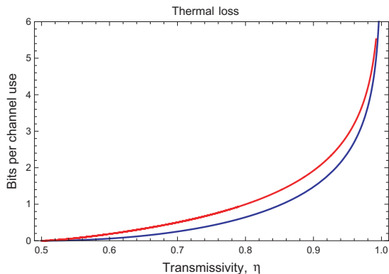
FIG. 1: Finite-resource bound \Psi(\mathcal{E}_{\eta, \bar{n}}) on the secret-key capacity of the thermal loss channel (red upper curve) as a function of the transmissivity \eta , compared with the infinite-energy bound \Phi(\mathcal{E}_{\eta, \bar{n}}) (blue lower curve) derived in Ref. [11]. The curves are plotted for \bar{n} = 1 thermal photons.
