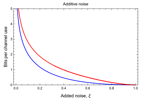
FIG. 3: Finite-resource bound \Psi(\mathcal{E}_\xi) on the secret-key capacity of the additive noise Gaussian channel (red upper curve) as a function of the added noise \xi , compared with the optimal bound for infinite energy \Phi(\mathcal{E}_\xi) (blue lower curve).
