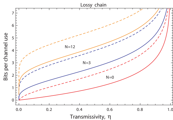
FIG. 5: Secret-key capacity of a chain of N equidistant repeaters creating N+1 pure-loss channels with transmissivities \eta_i = \frac{\eta}{N+1} . We compare the finite-resource bound (dashed) with the infinite-energy bound (solid) for different values of N as a function of the overall transmissivity of the chain \eta .
