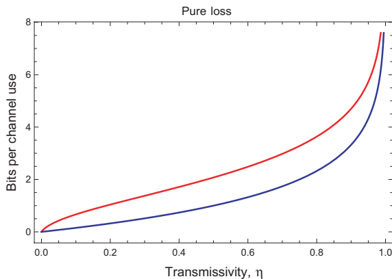
FIG. 4: Finite-resource bound \Psi(\mathcal{E}_\eta) on the secret-key capacity of the pure-loss channel (red upper curve) as a function of the transmissivity \eta , compared with its secret key capacity or PLOB bound K(\eta) = -\log_2(1 - \eta) (blue lower curve).
