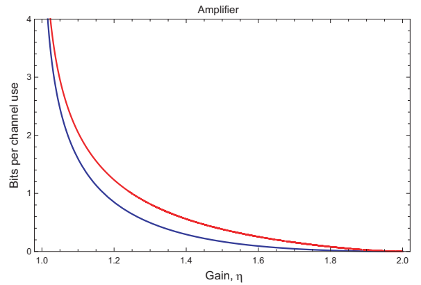
FIG. 2: Finite-resource bound \Psi(\mathcal{E}_{\eta, \bar{n}}) on the secret-key capacity of the noisy amplifier channel (red upper curve) as a function of the gain \eta , compared with the optimal bound for infinite energy \Phi(\mathcal{E}_{\eta, \bar{n}}) (blue lower curve). The two curves are plotted for \bar{n} = 1 thermal photons.
