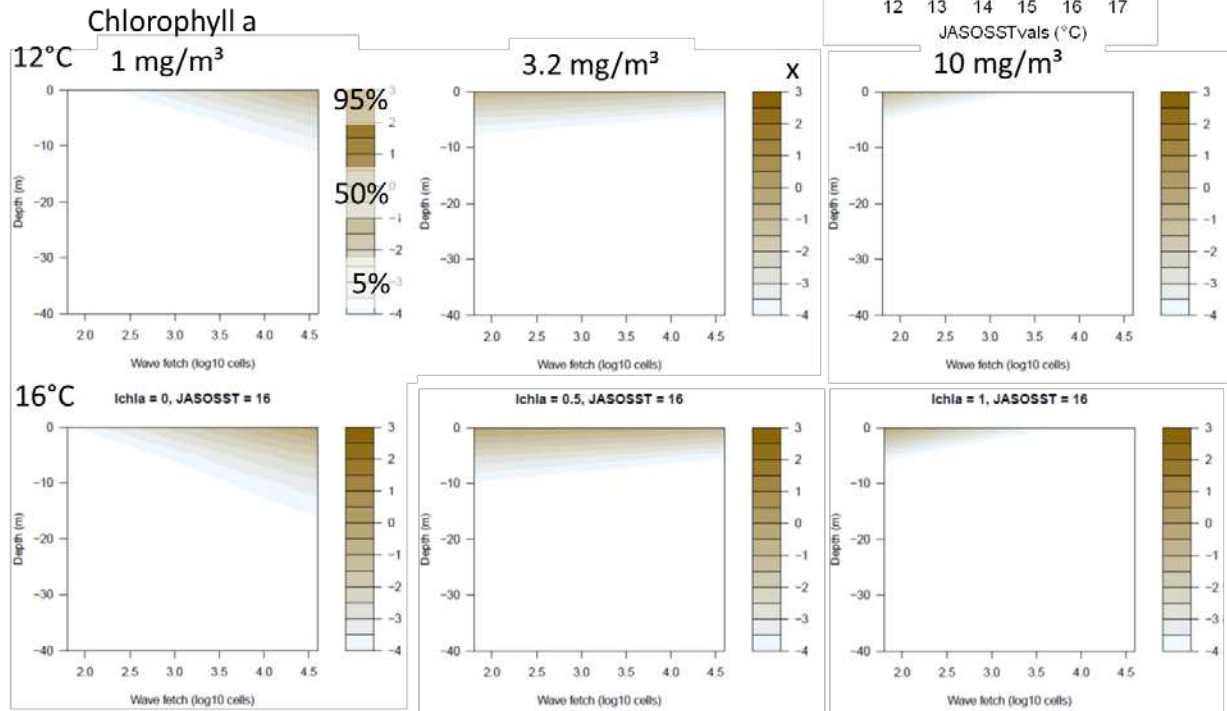
Figure A3. Habitat suitability model for Laminaria digitata . As in Fig. A1, intensity of brown shading shows likelihood of presence across gradients of depth (vertical) and wave exposure (horizontal) at different temperatures and chlorophyll concentrations.
