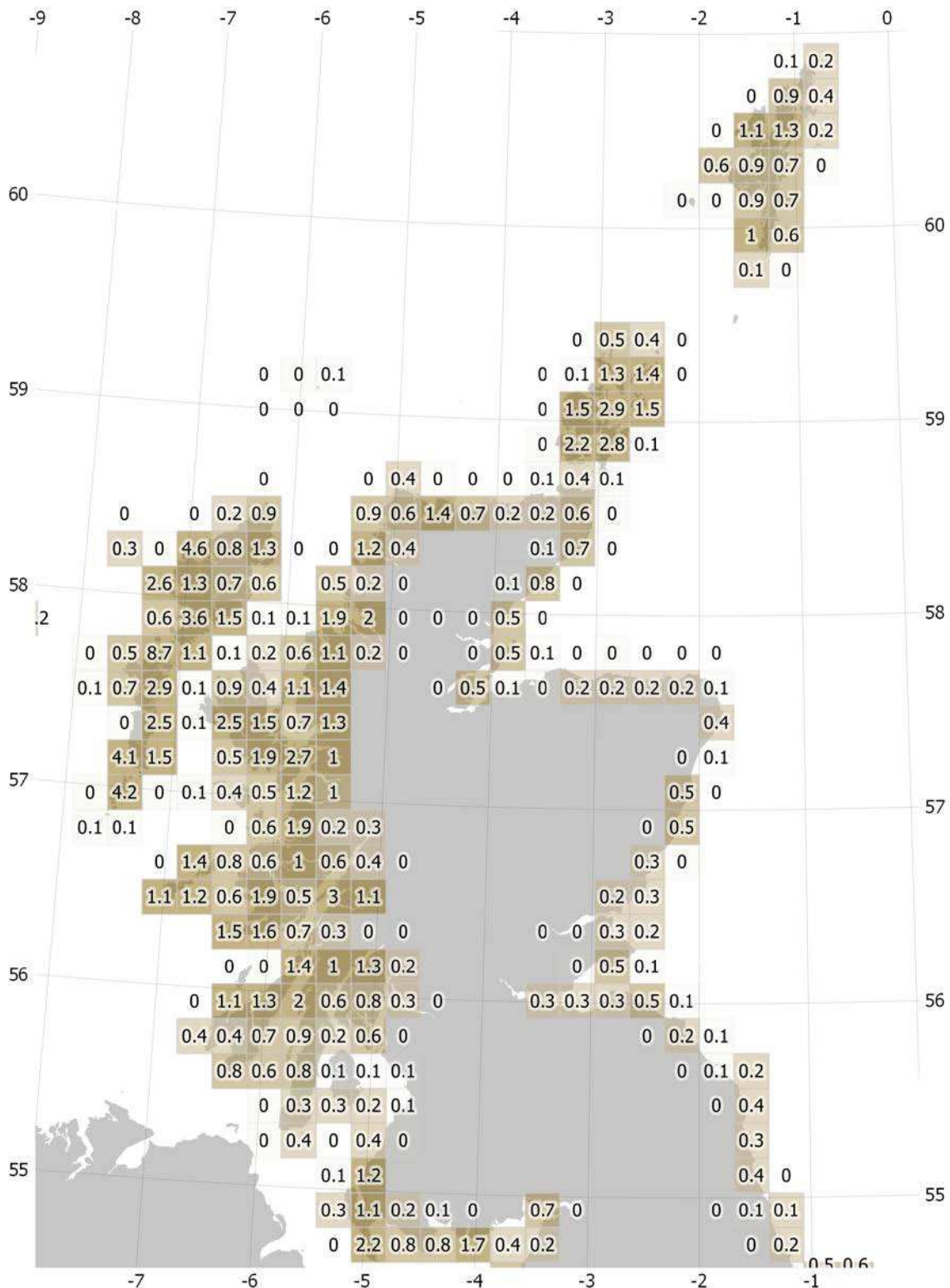
Figure 10. Predicted biomass of Laminaria digitata (in 1,000 tonne units) across all biomass densities by 20 km grid squares around Scotland.
