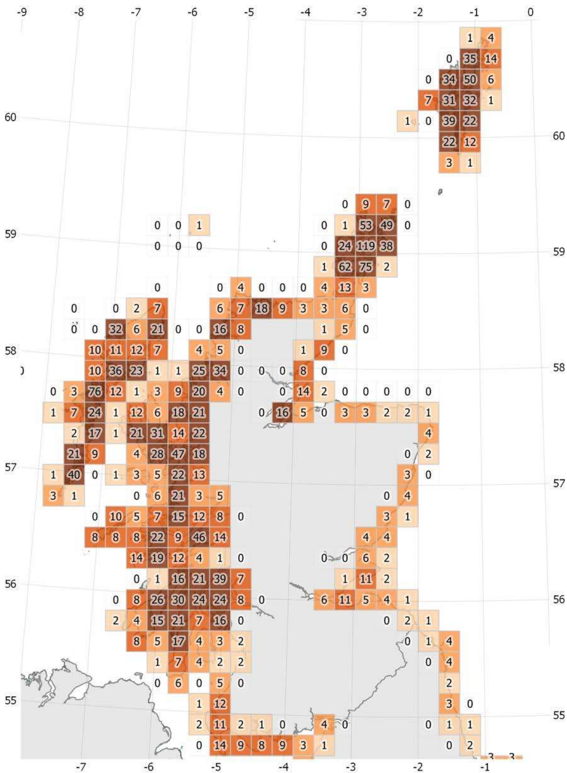
Figure 8. Predicted biomass of Saccharina latissima (in 1,000 tonne units) across all biomass densities by 20 km grid squares around Scotland.
