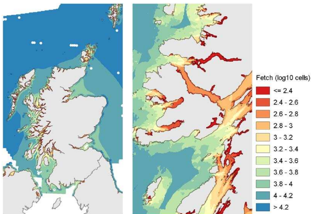
Figure 1. Wave fetch (left) around Scotland, and (right) in W Scotland showing wave-exposed (blue) and wave-sheltered areas (red), typical of Laminaria hyperborea and Saccharina latissima habitats respectively.
