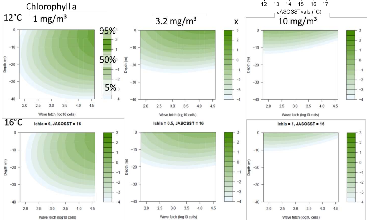
Figure A1. Habitat suitability model for Laminaria hyperborea . Intensity of green shading shows likelihood of presence across gradients of depth (vertical) and wave exposure (horizontal) at different temperatures and chlorophyll concentrations.
