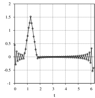
(i) \varepsilon = 0 , \gamma(\varepsilon) = 10^{-3} .
