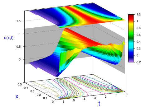
(c) U^\varepsilon(x, t), \gamma(\varepsilon) = 10^{-2}
