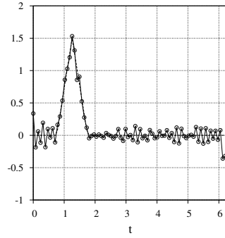
(b) \varepsilon = 2 \times 10^{-2} , \gamma(\varepsilon) = 10^{-2} .
