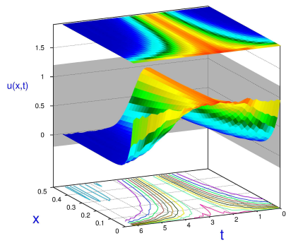
(b) u^\varepsilon(x, t), \gamma(\varepsilon) = 10^{-2}
