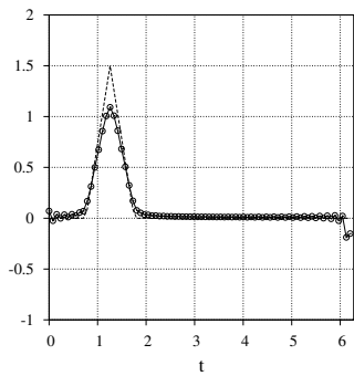
(g) \varepsilon = 0 , \gamma(\varepsilon) = 10^{-1} .
