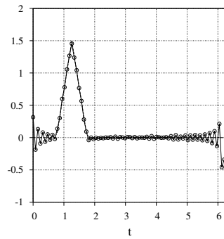
(e) \varepsilon = 2 \times 10^{-3} , \gamma(\varepsilon) = 10^{-2} .
