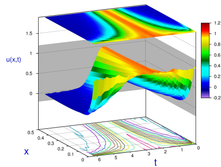
(e) U^\varepsilon(x, t), \gamma(\varepsilon) = 10^{-3}
