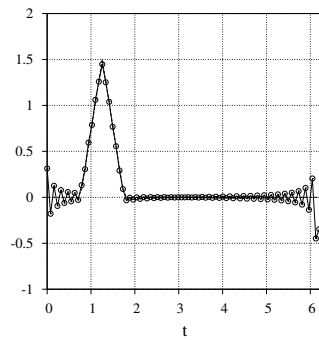
(h) \varepsilon = 0 , \gamma(\varepsilon) = 10^{-2} .
