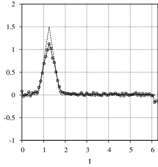
(a) \varepsilon = 2 \times 10^{-2} , \gamma(\varepsilon) = 10^{-1} .
