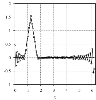
(f) \varepsilon = 2 \times 10^{-3} , \gamma(\varepsilon) = 10^{-3} .
