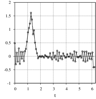
(c) \varepsilon = 2 \times 10^{-2} , \gamma(\varepsilon) = 10^{-3} .
