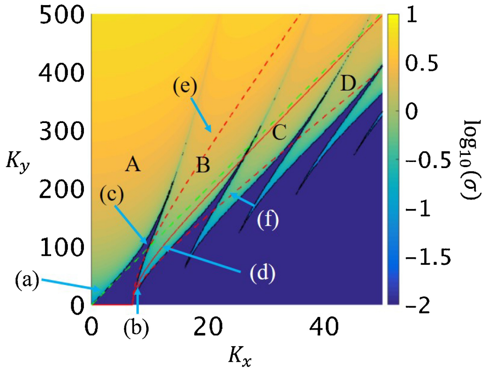
Figure 3. Numerically computed logarithm of the growth rate in K -space. Blue regions are approximately stable (with \sigma \leq 10^{-2} ). The top left-hand region (which emanates from K_x = K_y = 0 ) is KH unstable, whereas the five fingers of instability (yellowish regions pointing down) to the right of the KH band (associated with K_x = p/\sqrt{2\alpha_+} for K_y = 0 ) are parametrically unstable. These fingers of instability are associated with p = 1-5 in equation (40). The capital letters A–D mark different instability bands, where A = KH instability, B = parametric ( p = 1 ), C = parametric ( p = 2 ), D = parametric ( p = 3 ). The green dashed line marks the critical wavenumber for the growth of the KH instability in the asymptotic limit. The solid red line gives the fastest growing parametric mode in the asymptotic limit, with the dashed red lines marking the band of approximate resonance valid for small K_y . In this calculation \alpha_+ = 0.01 and M_A = 0.2 . The labelled blue arrows show the position in K -space of the six calculations shown in Fig. 2.
