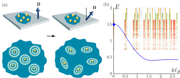
FIG. 1. (a) Geometric quench protocol: instantaneous tilt of the magnetic field induces dynamics of the intrinsic metric, which describes the shape of particle-flux composites that form a FQH state. (b) The excitation spectrum of the \nu = 1/3 Laughlin state, obtained by exact diagonalization of its V_1 parent Hamiltonian, in systems with N = 7 - 10 electrons. Blue line traces out the SMA collective mode [60], which transforms into an emergent graviton excitation in the k \rightarrow 0 limit (around energy E \approx 1.5 ). It will be shown in Sec. V that geometric quench induces oscillatory dynamics of the k \rightarrow 0 limit of the graviton mode. Note that this mode is formed by excited states in the continuum of the energy spectrum.
