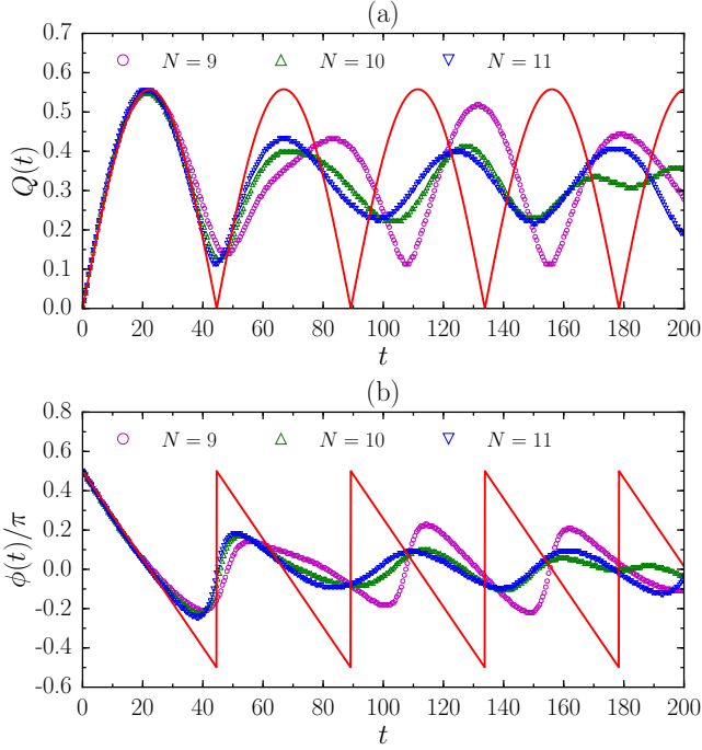
FIG. 13. Exact dynamics of (a) Q and (b) \phi for N = 9 - 11 fermions at \nu = 1/3 with the Coulomb interaction. The weak geometric quench is driven by choosing A_0 = 0 and A_1 = \ln 2.0 . The red solid curve is the Q \geq 0 part of Eqs. (5) and (6), with A \approx 0.279 and E_\gamma \approx 0.141 . These two parameters are obtained by fitting the first oscillation of Q of N = 11 against the solution.
