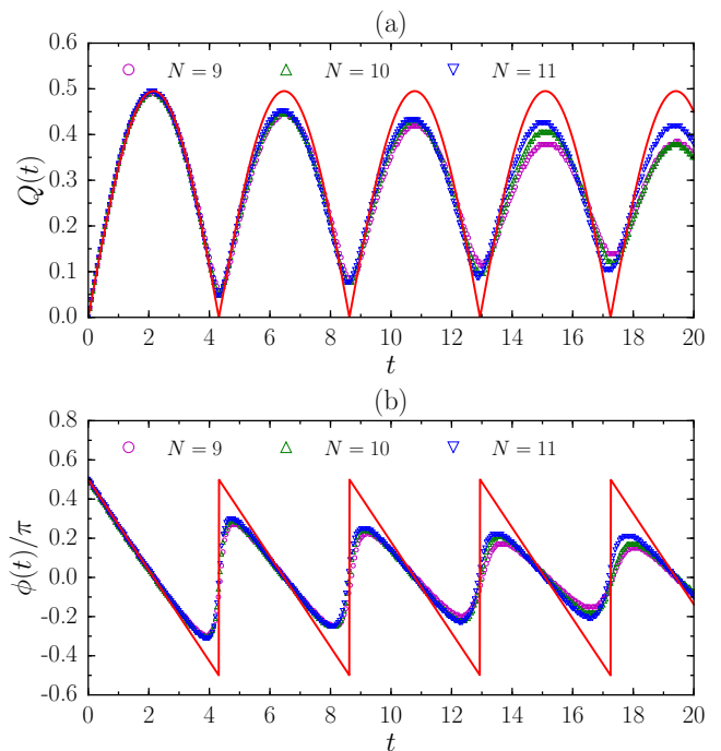
FIG. 12. Exact dynamics of (a) Q and (b) \phi for N = 9 - 11 fermions at \nu = 1/3 with the V_1 interaction. The weak geometric quench is driven by choosing A_0 = 0 and A_1 = \ln 1.3 . The red solid curve is the Q \geq 0 part of Eqs. (5) and (6), with A \approx 0.248 and E_\gamma \approx 1.457 . These two parameters are obtained by fitting the first oscillation of Q of N = 11 against the solution.
