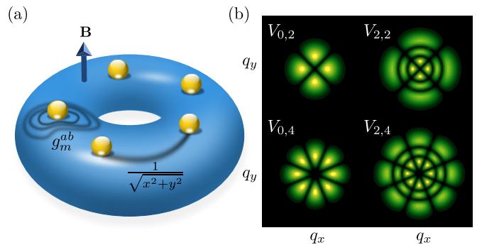
FIG. 2. (a) A FQH system on the surface of a torus threaded by perpendicular magnetic field. The mass tensor g_m determines the metric of the Landau level orbitals and is used to drive a quench, while the Coulomb potential is assumed to be isotropic. (b) Contours in momentum space of the leading order anisotropic pseudopotentials for bosons [51] with quadrupolar ( V_{0,2} , V_{2,2} ) and octupolar ( V_{0,4} , V_{2,4} ) structure.
