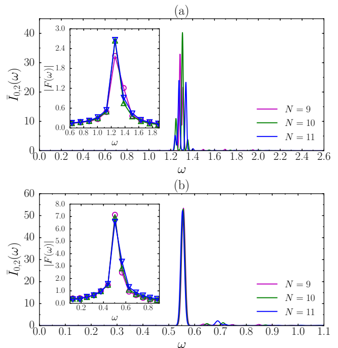
FIG. 5. Normalized spectral function \bar{I}_{0,2}(\omega) = I_{0,2}(\omega) / \int I_{0,2}(\omega)d\omega for isotropic systems of N = 9 - 11 bosons at \nu = 1/2 with (a) contact and (b) Coulomb interactions. The insets show the discrete Fourier transform |F(\omega)| of Q in Figs. 3 and 4. Markers in insets and curves in main figures with the same color refer to the same system size.
