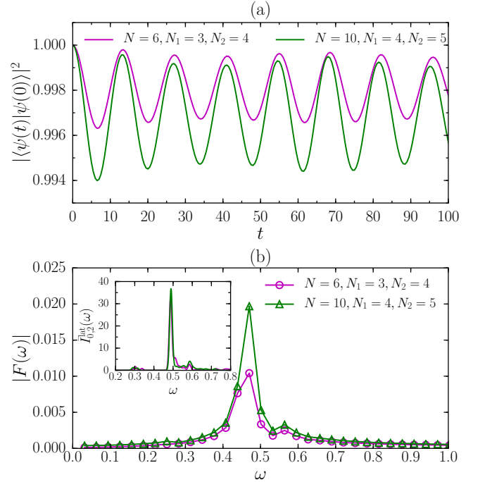
FIG. 14. (a) Dynamics of fidelity, |\langle \psi(t) | \psi(0) \rangle|^2 , and (b) its discrete Fourier transform for \nu = 1/2 bosonic Laughlin FCIs. The weak quench is driven by \alpha' = 15^\circ . The inset of (b) shows the normalized spectral function \bar{I}_{0,2}^{\text{lat}}(\omega) = I_{0,2}^{\text{lat}}(\omega) / \int I_{0,2}^{\text{lat}}(\omega) d\omega for the isotropic case with \alpha = 0 . Markers in insets and curves in main figures with the same color refer to the same system size.
