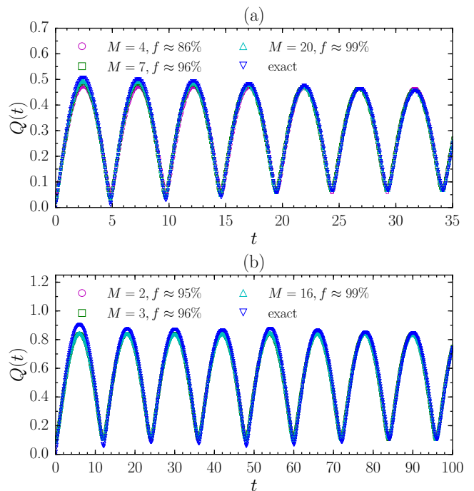
FIG. 10. Dynamics of Q projected to M eigenstates of H' with dominant |\langle n | \hat{V}_{0,2} | 0 \rangle|^2 . We consider N = 11 bosons with (a) contact and (b) Coulomb interactions. The quench parameters A_0 and A_1 are the same as those in Figs. 3 and 4, respectively.
