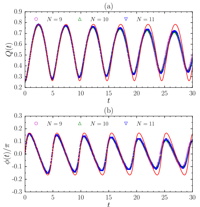
FIG. 9. Exact dynamics of (a) Q and (b) \phi for N = 9 - 11 bosons at \nu = 1/2 with the contact interaction. The weak geometric quench is driven by choosing A_0 = \ln 1.3 and A_1 = \ln 1.7 . The red solid curve is the solution of linearized equations Eqs. (20) and (21) under the initial condition Q(0) = A_0, \phi(0) = 0 , with A \approx 0.523 and E_\gamma \approx 1.283 . These two parameters are obtained by fitting the first oscillation of Q of N = 11 against the solution.
