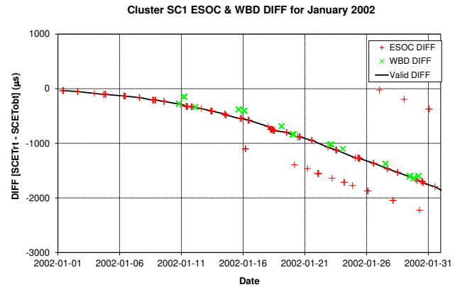
Fig. 1. Plot of the DIFF values measured by ESOC (+) and WBD ( \times ). The solid line represents the assumed correct value used to prepare the time corrections. The “DIFF” (the difference between the ground receive time and the onboard time) is measured during every ground station contact. However some measurements are subject to errors, so a validation process must be applied.
