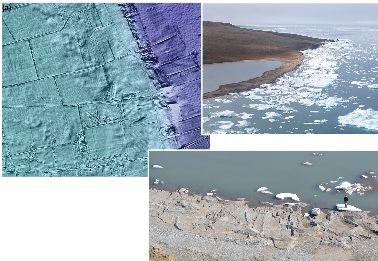
Figure 11. Landforms on the southern Vale of York/Humber lowlands and probable modern analogues: (a) LiDAR image showing overprinted hummocky and arcuate ridges at the Wolds scarp footslope and examples of the most likely modern analogues of floating ice push ridges on the coast of Banks Island, Arctic Canada; (b) LiDAR image showing, at the top, discontinuous sinuous ridges connecting with oval to circular rimmed depressions and, at the base, dual ridged polygonal forms. Examples of modern analogues from recently drained, aggrading permafrost terrains in Arctic Canada are depicted at right, with the upper images showing ice wedge and pingo complexes from Banks Island, and the lower images showing ice wedge landforms from northern Ellesmere Island.
