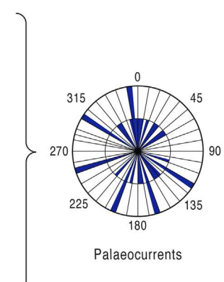
Figure 4. Composite vertical profile log (a) and clast lithologies for selected facies (b) from the exposure at North Cave. The log shows major lithofacies and the internal structures, clast form and palaeocurrent data (based on downflow dip directions of avalanche or lee side beds in cross-bedded sands), and locations of OSL and ^{14}C dates. Inset photograph shows the nature of syngenetic ice wedge pseudomorphs developed in the base of LF4a and extending down into LF3 and LF2.
