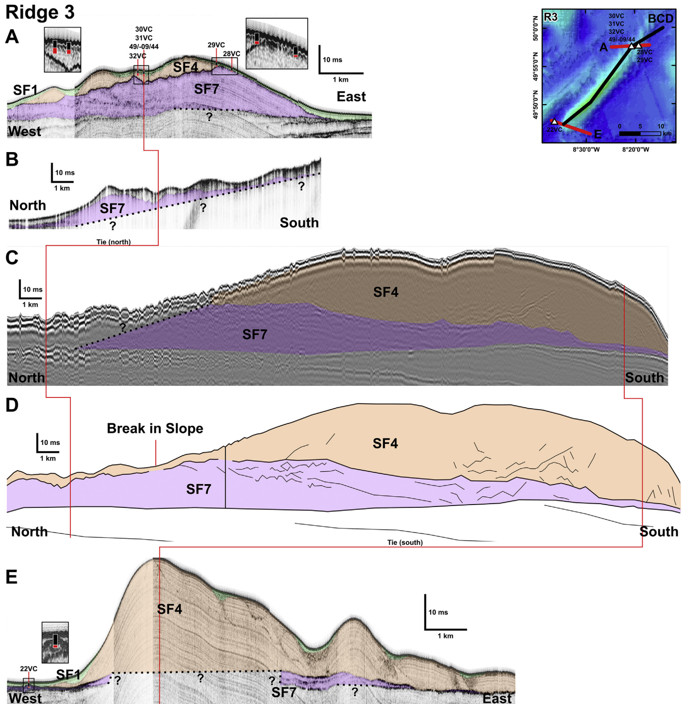
Fig. 4. Seismic-facies based on chirp (A, B and E) and sparker (C) data of Ridge 3 with D showing the combination of B and C along the crest with the merge point marked. See Fig. 1 for line and inset locations.
