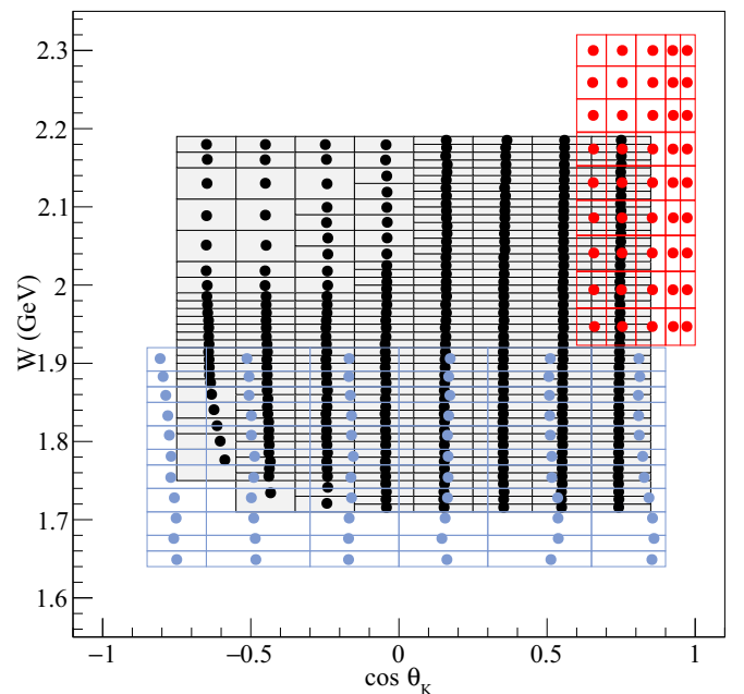
FIG. 3. Comparison of kinematic coverage in W vs \cos \theta_K^* for \bar{\nu}p \rightarrow K^+\bar{\Lambda} . Black circles: this (CLAS) measurement; red circles: LEPS; blue circles - GRAAL. The boxes represent the limits of the bins in \{W, \cos \theta_K^*\} .
