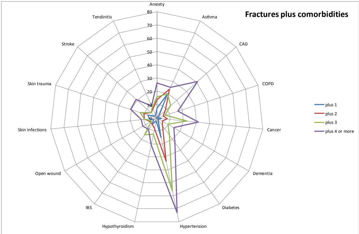
Figure 33 Top 15 most frequent co-morbidities for those with fractures
