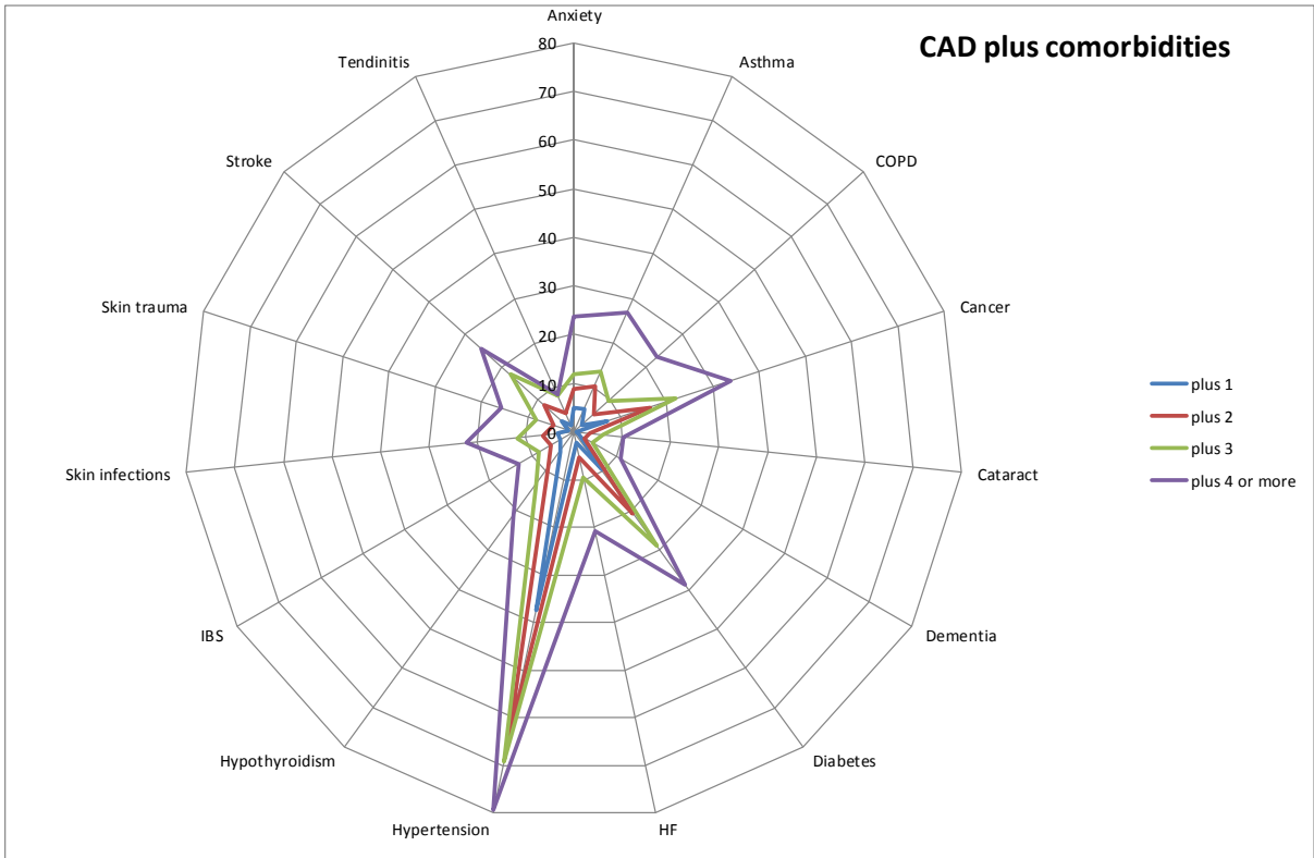
Figure 35 Top 15 most frequent co-morbidities for those with CAD
