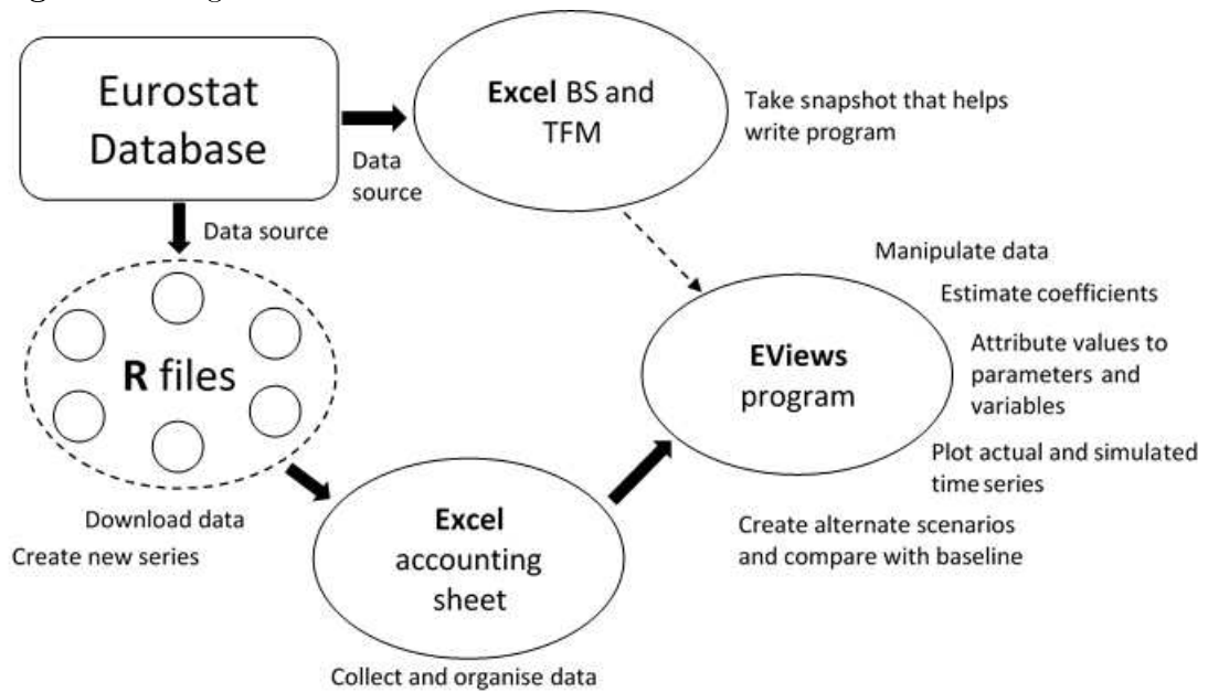
Figure 6: Programs' structure
