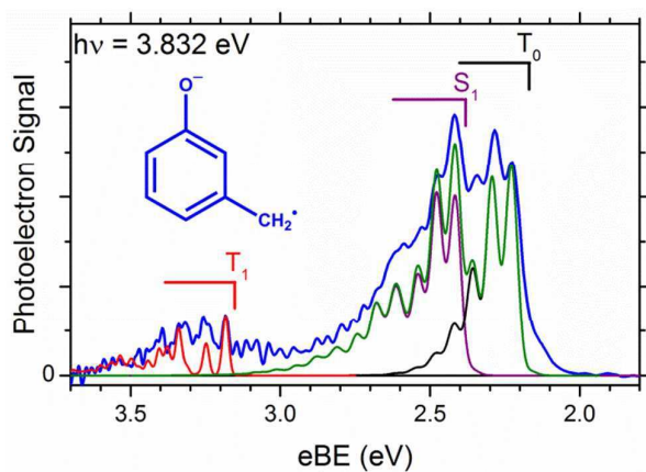
Fig. 7 Photoelectron spectra of m/z = 106 , resulting from the reaction of \text{O}^- with m -methylphenol, collected with the pulsed PES instrument using a photon energy of 3.832 eV (blue trace). The PES simulations, convolved with the experimental resolution, are shown as black, purple, and red lines for transitions to the neutral T_0 , S_1 , and T_1 electronic states, respectively, from the ground state of the m -methylenephenoxy anion. The sum of the simulated PES in the 2 – 3 eV range is shown as the green line.
