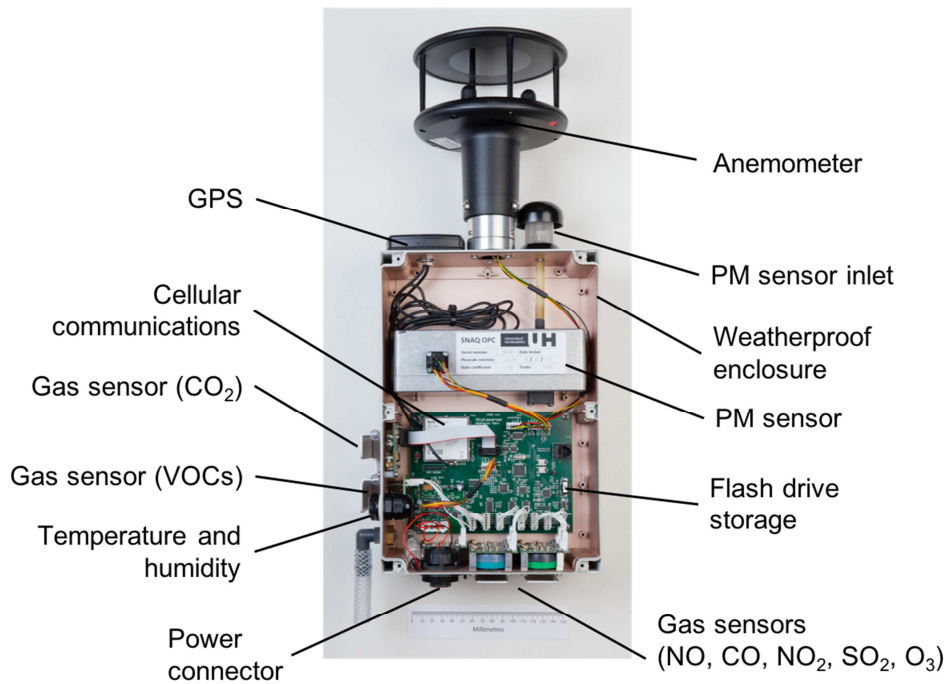
Figure 2. Sensor system showing enclosure, sensors, and supporting hardware
