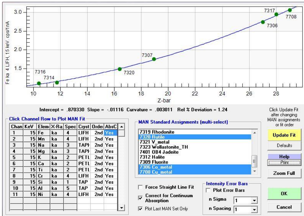
Figure 8. A mean atomic number plot showing background intensity across a range of different values of mean atomic number ( \bar{z} -bar).
