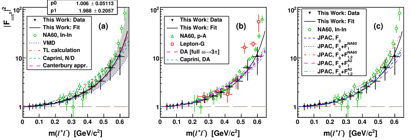
FIG. 19: (Color online) |F_{\omega\pi^0}(m_{\ell^+\ell^-})|^2 results (black filled triangles) combined from Run-I and Run-II and their pole-approximation fit (black solid line, with p_0 and p_1 being the normalization and the slope parameter \Lambda^{-2} , respectively) are compared to previous measurements and various theoretical calculations. The results by Lepton-G [23] are shown by open red squares in panel (b). The results of NA60 obtained in peripheral In-In data [15] are shown by open green circles in (a) and (c), and from p-A collisions [12] by open green triangles in (b). The VMD prediction is shown by a blue dashed line in (a). The calculation from Refs. [24, 25] is shown by a red dash-dotted line in (a). The DA calculation by the Bonn group [26] for the full 3\pi rescattering is shown by error-band borders (magenta dashed lines) in (b). Upper and lower bounds by Caprini [30] are shown by cyan dashed lines for two cases of the discontinuity calculated with the partial-wave amplitude f_1(t) based on the improved N/D model [52] (a), and taken from Ref. [26] (b). The calculation based on a model-independent method using Canterbury approximants [53] is shown by a magenta long-dashed line with a gray error band. The basic calculation (blue dashed line) from JPAC [27] and the effect from including higher order terms of the inelastic contributions in the \omega\pi^0 TFF by fitting them to the NA60 In-In data is shown in (c) for the solutions with adding one (black dotted line) and two (red dash-dotted line) terms. A similar effect from including higher order terms by fitting them to the present |F_{\omega\pi^0}(m_{\ell^+\ell^-})|^2 results is shown in (c) for the solutions with one (magenta long-dashed line) and with two (cyan dash-double-dotted line) terms.
