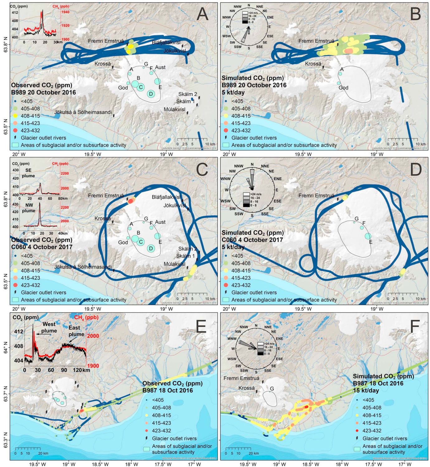
Figure 2. Observed and simulated CO 2 plumes from Katla volcano on 18 and 20 October 2016 and 4 October 2017. The panels show the wind direction and speed measured during each flight and along-track points of CO 2 and CH 4 concentrations. (a) Observed CO 2 peak on 20 Oct 2016 (flight B989). (b) The best-fit simulated sources for the CO 2 peak observed on 20 Oct 2016: rivers Fremri Emstruá and Krossá, ice cauldron cluster A, and Goðabunda rise. The figure shows simulation of 5 kt/d of CO 2 , but good agreement was also reached with 10 kt/d. (c) Two observed CO 2 peaks on 4 Oct 2017 (flight C060), to the northwest (NW) and southeast (SE) of the caldera. (d) The best-fit simulated sources for the CO 2 peaks observed on 4 Oct 2017: river Fremri Emstruá and ice cauldron clusters E, F and G. The figure shows simulation of 5 kt/d of CO 2 , but good agreement was also reached with 10 kt/d. (e) Two observed CO 2 peaks on 18 Oct 2016 (flight B987), to the west and east of the caldera. (f) The best-fit simulated sources for the CO 2 peaks observed on 18 Oct 2016—rivers Fremri Emstruá and Krossá and ice cauldron cluster G. Both of the observed CO 2 peaks can be traced to Katla when CO 2 is simulated as a dense gas with emission rate of 15 kt/d.
