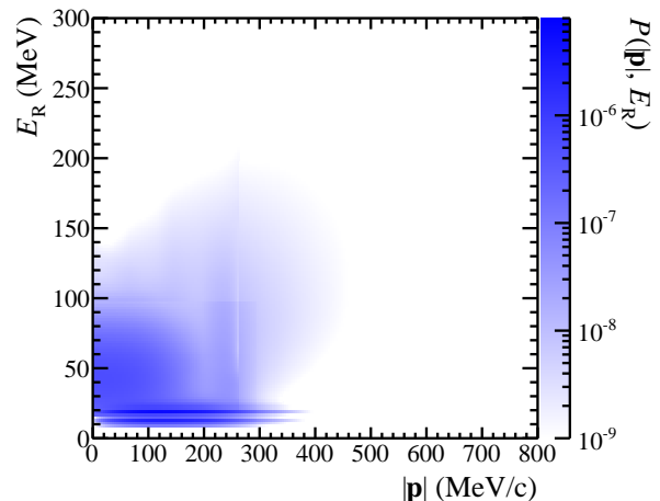
FIG. 1: The probability distribution for initial state protons within an oxygen nucleus for Benhar's SF model [23] as a function of the removal energy ( E_R ) and the magnitude of the nucleon momentum ( |\mathbf{p}| ). The SF is normalized such that the integral of this distribution is 1.
