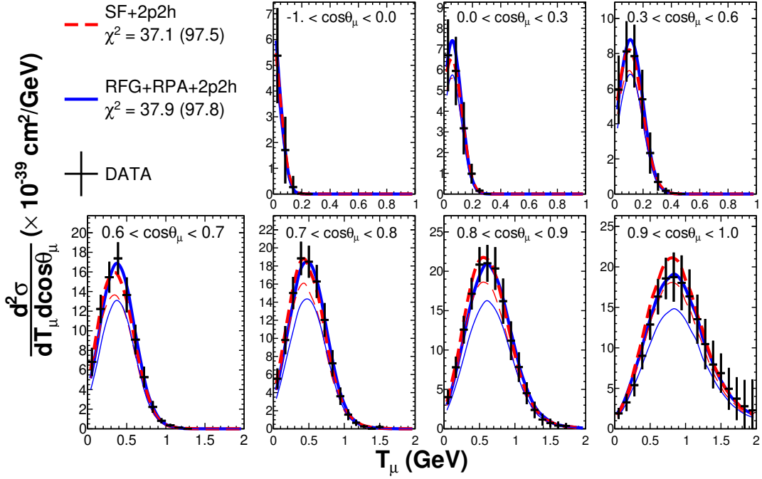
(a) Neutrino
