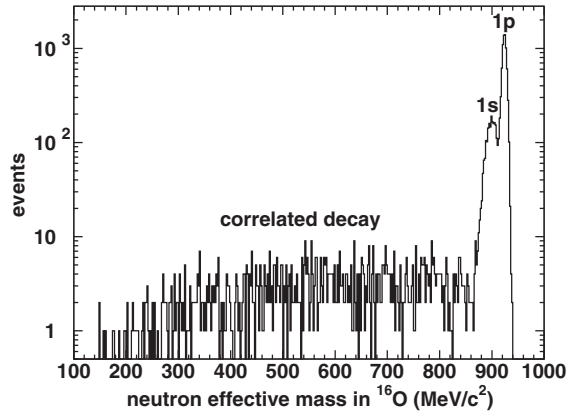
FIG. 1. The effective mass of the decayed neutron in ^{16}\text{O} for n \rightarrow e^+\pi^- as simulated by Monte Carlo.
