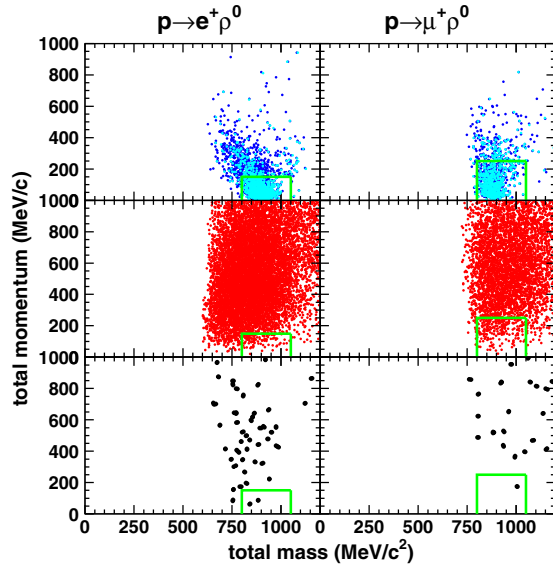
FIG. 10. Total invariant mass and total momentum for p \rightarrow l^+\rho^0 MC (top, cyan for free proton and blue for bound proton), atmospheric neutrino background MC corresponding to about 2000 years live time of SK (middle), and data (bottom) for p \rightarrow e^+\rho^0 (left) and p \rightarrow \mu^+\rho^0 (right) searches. All the event selections except (C5) in Sec. IV B are applied. The results from SK-I to SK-IV are combined. The signal box is shown as a green box.
