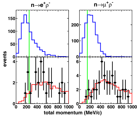
FIG. 21. Total momentum for n \rightarrow l^+ \rho^- MC (upper), atmospheric neutrino MC (lower, red histogram), and data (lower, black circles) for n \rightarrow e^+ \rho^- (left) and n \rightarrow \mu^+ \rho^- (right) searches. All the event selections except (G6) in Sec. IV E are applied. The atmospheric neutrino MC is normalized to data by area. Results from SK-I to SK-IV are combined. The signal region corresponds to the left side from the vertical green line. Total momenta of the data candidates are 173 MeV/c, 235 MeV/c, 239 MeV/c, 246 MeV/c for n \rightarrow e^+ \rho^- search and 129 MeV/c for n \rightarrow \mu^+ \rho^- search.
