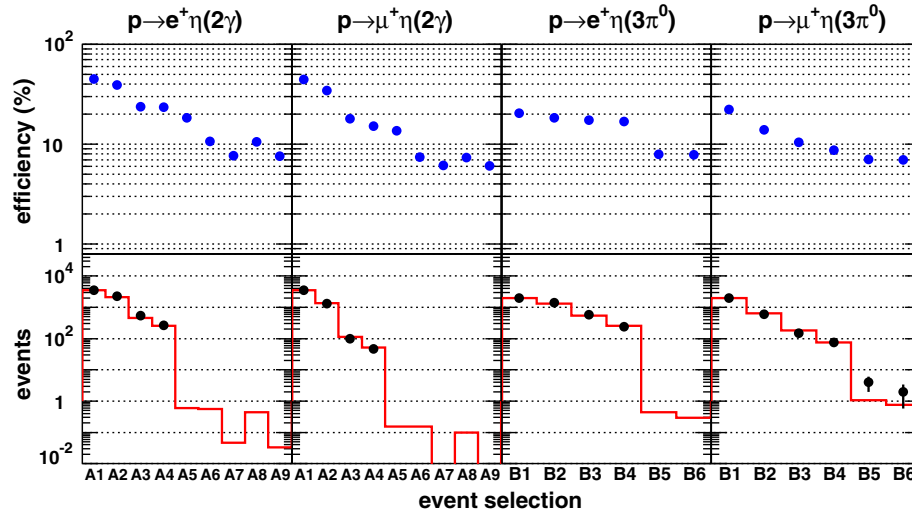
FIG. 6. The signal efficiencies (upper) and the number of expected backgrounds (lower, red histogram) and data candidates (lower, black dots) for p \rightarrow e^+\eta ( \eta \rightarrow 2\gamma ), p \rightarrow \mu^+\eta ( \eta \rightarrow 2\gamma ), p \rightarrow e^+\eta ( \eta \rightarrow 3\pi^0 ), and p \rightarrow \mu^+\eta ( \eta \rightarrow 3\pi^0 ) searches from left to right. The results from SK-I to SK-IV are combined. The event selection is defined in the text.
