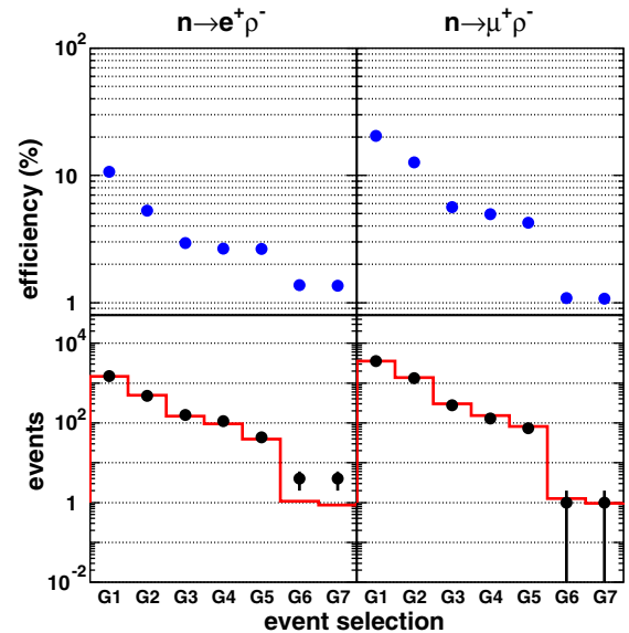
FIG. 19. The signal efficiencies (upper) and the number of expected backgrounds (lower, red histogram) and data candidates (lower, black dots) for n \rightarrow e^+ \rho^- (left) and n \rightarrow \mu^+ \rho^- (right). The results from SK-I to SK-IV are combined. The event selection is defined in the text.
