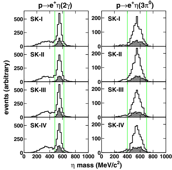
FIG. 5. The reconstructed \eta mass distributions for p \rightarrow e^+\eta MC events for \eta \rightarrow 2\gamma search (left) and \eta \rightarrow 3\pi^0 (right) search for each SK period. The histograms show all simulated p \rightarrow e^+\eta events. For the left plots the eta meson is reconstructed under the assumption of \eta \rightarrow 2\gamma , and for the right plots the eta meson is reconstructed under the assumption of \eta \rightarrow 3\pi^0 . The hatched histograms show, for free proton decays, the true \eta \rightarrow 2\gamma events (left) and true \eta \rightarrow 3\pi^0 events (right). The event selections (A1–A2) of Sec. IV A are applied. The inside of the two vertical green lines corresponds to the signal region.
