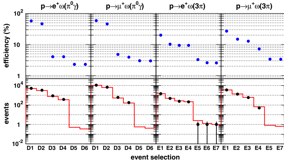
FIG. 12. The signal efficiencies (upper) and the number of expected backgrounds (lower, red histogram) and data candidates (lower, black dots) for p \rightarrow e^+\omega ( \omega \rightarrow \pi^0\gamma ), p \rightarrow \mu^+\omega ( \omega \rightarrow \pi^0\gamma ), p \rightarrow e^+\omega ( \omega \rightarrow 3\pi ), and p \rightarrow \mu^+\omega ( \omega \rightarrow 3\pi ) searches from left to right. The results from SK-I to SK-IV are combined. The event selection is defined in the text.
