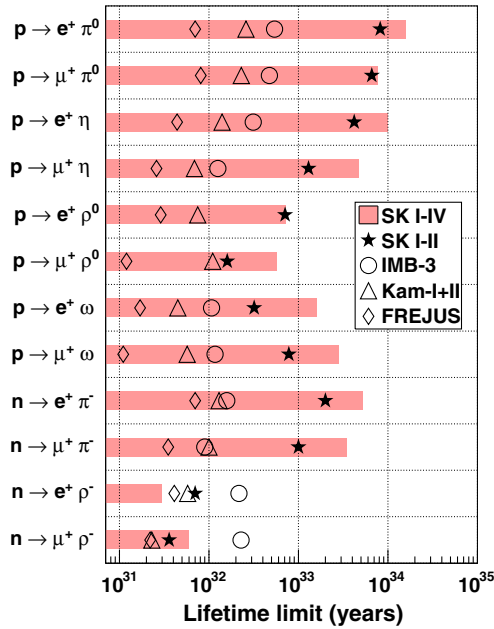
FIG. 22. Explored ranges and lower limits of nucleon partial lifetime with the results of the other experiments [27–29] and the previous SK analysis [11]. The p \rightarrow l^+ \pi^0 results [7] are also included.
