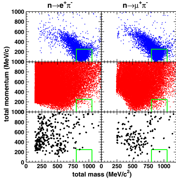
FIG. 17. Total invariant mass and total momentum for n \rightarrow l^+ \pi^- MC (top), atmospheric neutrino background MC corresponding to about 2000 years live time of SK (middle), and data (bottom) for n \rightarrow e^+ \pi^- (left) and n \rightarrow \mu^+ \pi^- (right) searches. All the event selections except (F4) in Sec. IV D are applied. The results from SK-I to SK-IV are combined. The signal region is shown as a green box.
