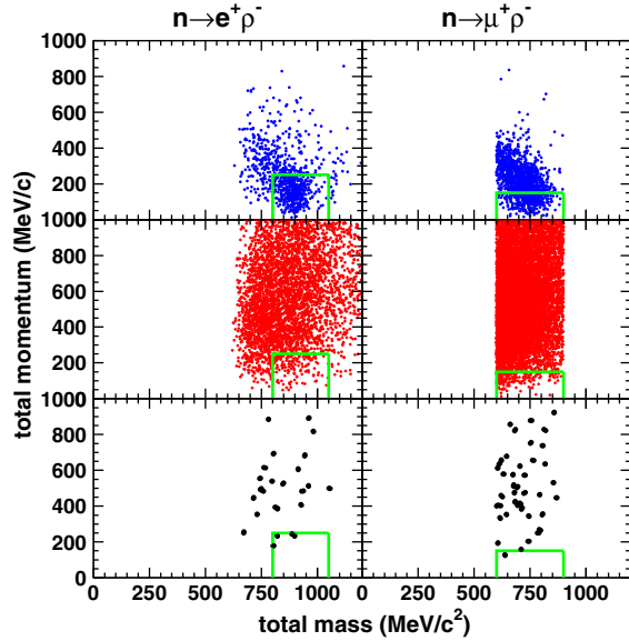
FIG. 20. Total invariant mass and total momentum for n \rightarrow l^+ \rho^- MC (top), atmospheric neutrino background MC corresponding to about 2000 years live time of SK (middle), and data (bottom) for n \rightarrow e^+ \rho^- (left) and n \rightarrow \mu^+ \rho^- (right) searches. All the event selections except (G6) in Sec. IV E are applied. The results from SK-I to SK-IV are combined. For the n \rightarrow e^+ \rho^- search, the signal box is shown as a green box. For the n \rightarrow \mu^+ \rho^- search, no total mass cut is applied in the analysis and the sharp cutoffs on the total mass correspond to the \rho^- mass cut threshold.
