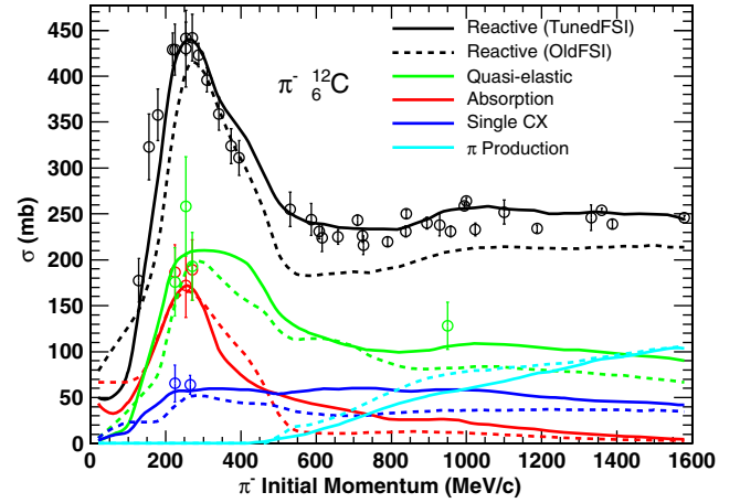
FIG. 2. The \pi^- interaction cross section on ^{12}\text{C} as a function of momentum. Open circles indicate existing data [18]; dashed and solid lines show before and after the tune, respectively. The colors correspond to the total cross section and exclusive channels: total (black), quasielastic scattering (green), absorption (red), charge exchange “CX” (blue), and \pi production (light blue). “FSI” stands for final state interaction.
