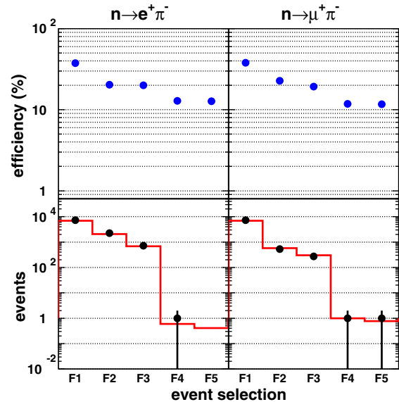
FIG. 16. The signal efficiencies (upper) and the number of expected background events (lower, red histogram) and data candidates (lower, black dots) for n \rightarrow e^+ \pi^- (left) and n \rightarrow \mu^+ \pi^- (right) searches. The results from SK-I to SK-IV are combined. The event selection is defined in the text.
