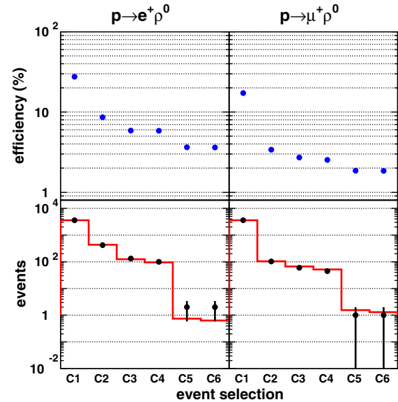
FIG. 9. The signal efficiencies (upper) and the number of expected backgrounds (lower, red histogram) and data candidates (lower, black dots) for p \rightarrow e^+ \rho^0 (left) and p \rightarrow \mu^+ \rho^0 (right) searches. The results from SK-I to SK-IV are combined. The event selection is defined in the text.
