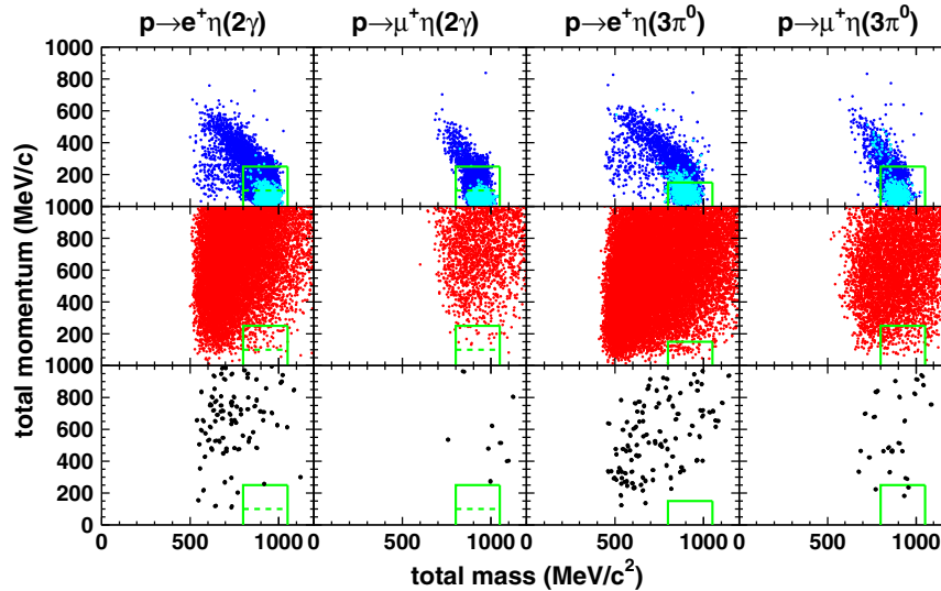
FIG. 7. Total invariant mass and total momentum for p \rightarrow l^+\eta MC (top, cyan for free proton and blue for bound proton), atmospheric neutrino background MC corresponding to about 2000 years live time of SK (middle), and data (bottom) for p \rightarrow e^+\eta ( \eta \rightarrow 2\gamma ), p \rightarrow \mu^+\eta ( \eta \rightarrow 2\gamma ), p \rightarrow e^+\eta ( \eta \rightarrow 3\pi^0 ), and p \rightarrow \mu^+\eta ( \eta \rightarrow 3\pi^0 ) searches from left to right. All the event selections except (A5–A7) and (B5) in Sec. IV A are applied. The results from SK-I to SK-IV are combined. The signal box is shown as a green box. For the p \rightarrow l^+\eta ( 2\gamma ) searches, the total momentum is separated at the horizontal dashed line in the signal box.
