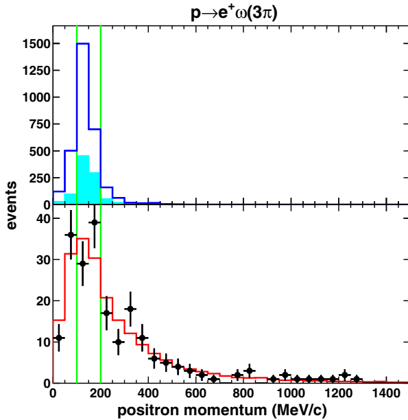
FIG. 15. Positron momentum for p \rightarrow e^+ \omega MC (upper, open histogram for bounded protons and shaded histogram for free protons), atmospheric neutrino MC (shaded, red histogram), and data (lower, black circles) for p \rightarrow e^+ \omega ( \omega \rightarrow 3\pi ) search. The event selections (E1–E4) of Sec. IV C are applied. The atmospheric neutrino MC is normalized to data by area. Results from SK-I to SK-IV are combined. The inside of the two vertical green lines corresponds to the signal region.
