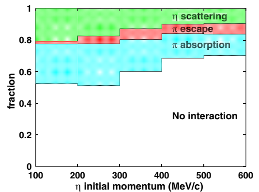
FIG. 3. Fraction of meson interactions in the oxygen nucleus in bins of \eta momentum generated by p \rightarrow e^+\eta MC. \eta 's that exit the nucleus without experiencing any interactions are indicated by the portion labeled “No interaction.” If at least one of the pions generated via the baryon resonance of N(1535) is absorbed, it is called “ \pi absorption.” If none of the pions are absorbed, it is called “ \pi escape.”
