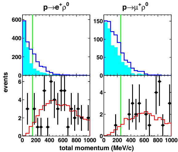
FIG. 11. Total momentum for p \rightarrow l^+\rho^0 MC (upper, open histogram for bounded protons and shaded histogram for free protons), atmospheric neutrino MC (lower, red histogram), and data (lower, black circles) for p \rightarrow e^+\rho^0 (left) and p \rightarrow \mu^+\rho^0 (right) searches. All the event selections except (C5) in Sec. IV B are applied. The atmospheric neutrino MC is normalized to data by area. Results from SK-I to SK-IV are combined. The signal region corresponds to left side from the vertical green line. Total momenta are 61 MeV/c and 90 MeV/c for the p \rightarrow e^+\rho^0 data candidates and 179 MeV/c for the p \rightarrow \mu^+\rho^0 data candidate.
