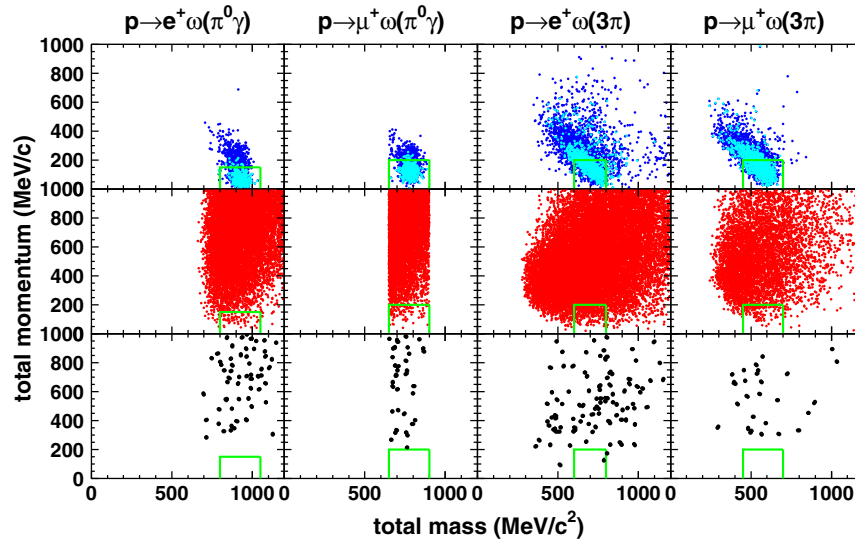
FIG. 13. Total invariant mass and total momentum for p \rightarrow l^+\omega MC (top, cyan for free proton and blue for bound proton), atmospheric neutrino background MC corresponding to about 2000 years live time of SK (middle), and data (bottom) for p \rightarrow e^+\omega ( \omega \rightarrow \pi^0\gamma ), p \rightarrow \mu^+\omega ( \omega \rightarrow \pi^0\gamma ), p \rightarrow e^+\omega ( \omega \rightarrow 3\pi^0 ), and p \rightarrow \mu^+\omega ( \omega \rightarrow 3\pi^0 ) searches from left to right. All the event selections except (D5) and (E5) in Sec. IV C are applied. The results from SK-I to SK-IV are combined. The signal box is shown as a green box.
