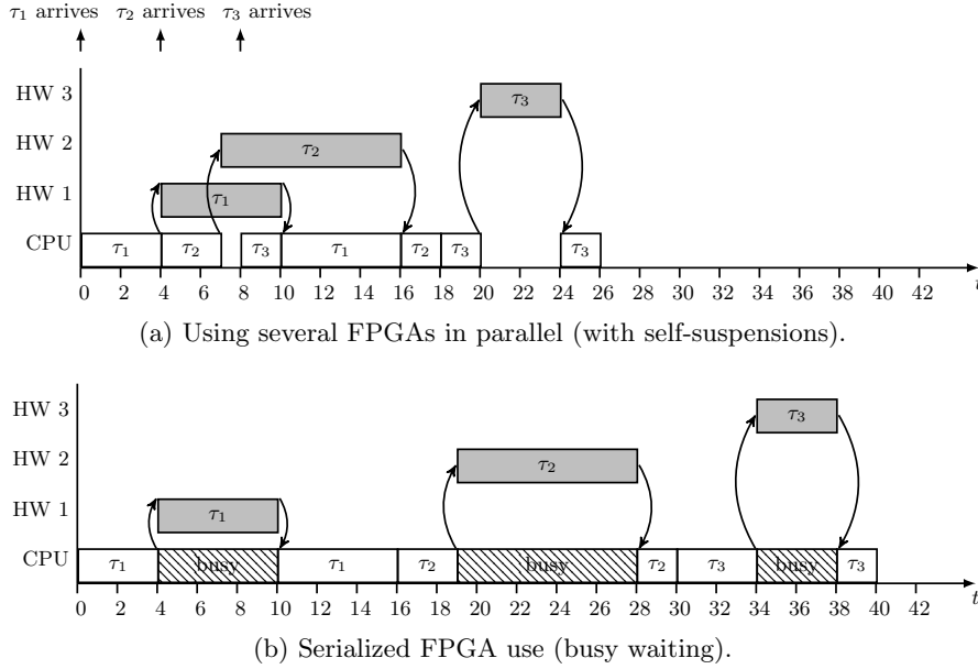
Fig. 2: An example of using FPGA for acceleration.
