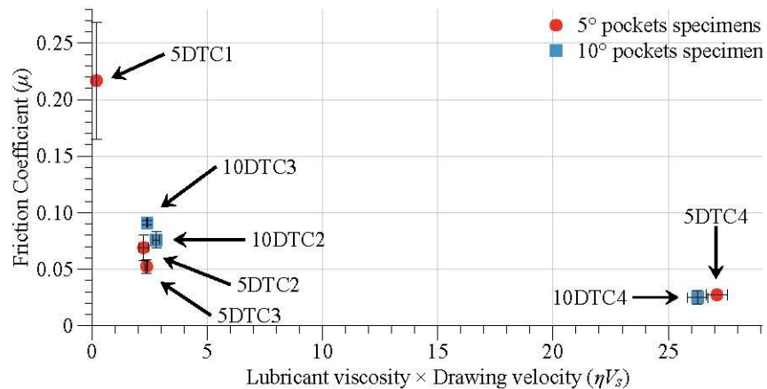
Figure 13: Evolution of the global friction coefficient according to the drawing velocity and lubricant viscosity, for each test configuration.
