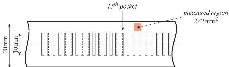
Figure 14: Location of measurements performed outside of the pockets row. row.
