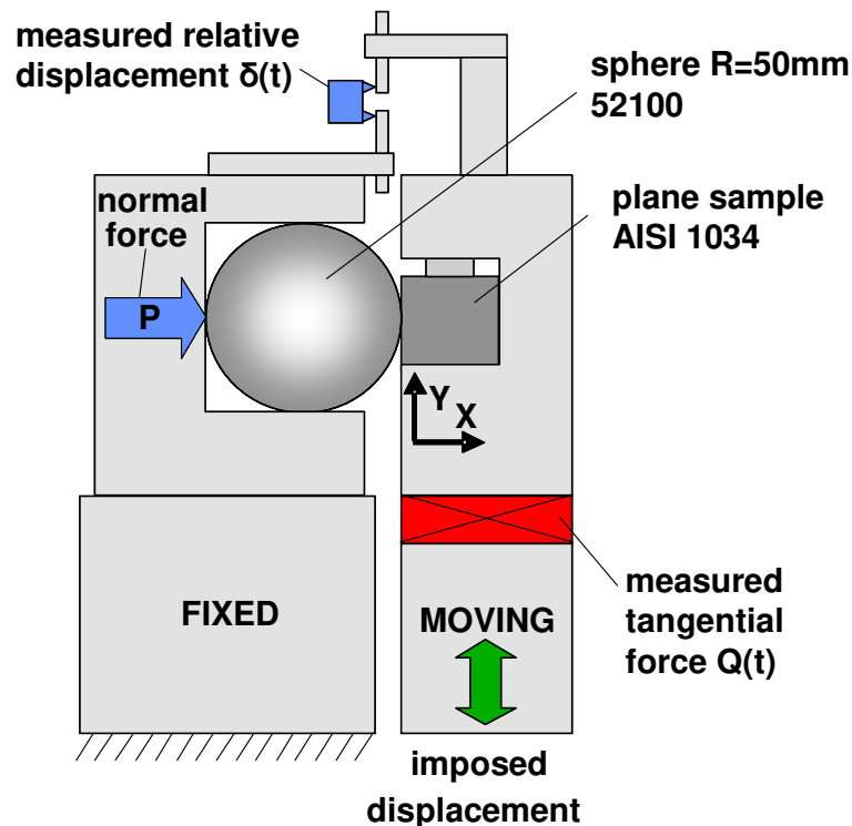
Fig. 3: Schematic diagram of fretting test device in sphere/plane configuration.
