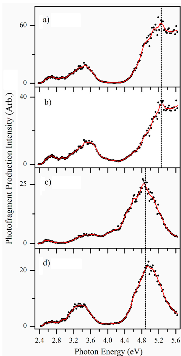
Figure 5. Photofragment action spectra of the fragments with (a) m/z 188, (b) m/z 144, (c) m/z 172 and (d) m/z 142 produced following photoexcitation of mass-selected \text{AL}\cdot\text{H}^+ ions, across the range 2.34–5.64 eV. The solid line is a three-point adjacent average of the data points.
