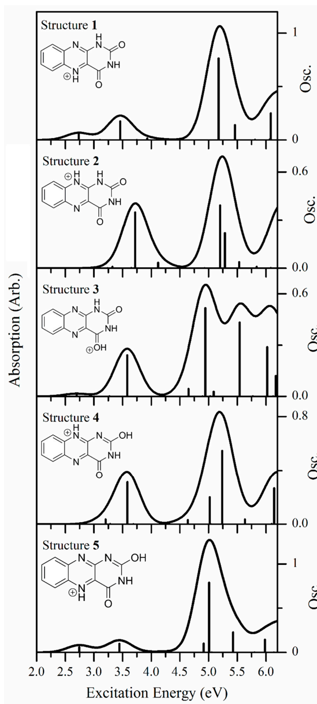
Figure 6. Calculated TDDFT excitation energies (with the PBE0 functional) of protomer 1, protomer 2, protomer 3, protomer 4, and protomer 5 of AL·H + . The oscillator strengths (abbreviated Osc. on the y axis) of individual transitions are given by the vertical bars, while the full line spectrum is a convolution of the calculated spectrum with a Gaussian function (0.25 eV HWHM).
