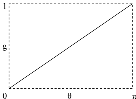
Figure 2: The invertible and continuous g -function g_1(\theta) = \theta/\pi .
