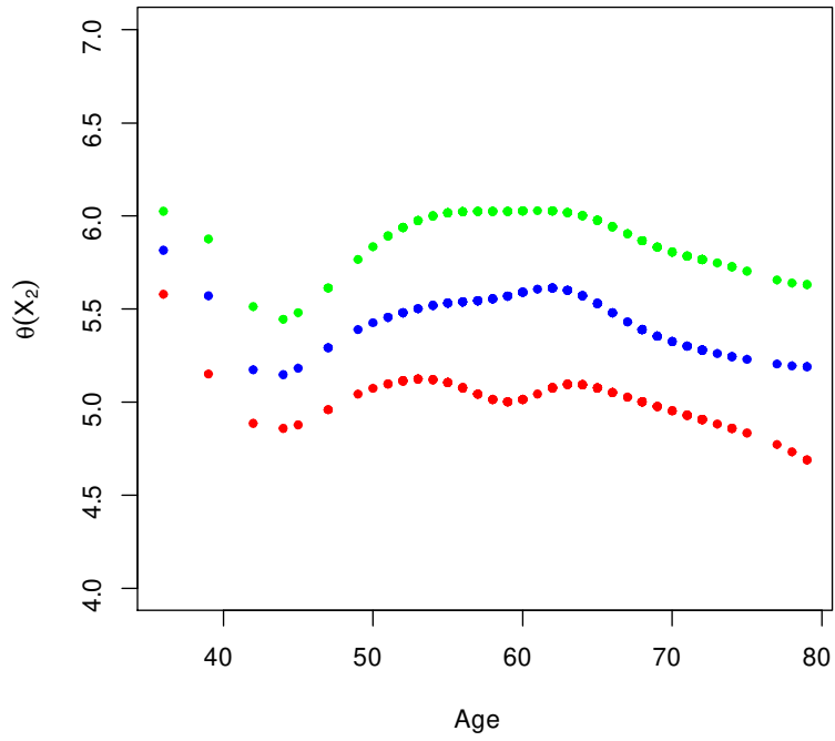
Figure 5. Nonparametric quantile estimates for \tau = (0.25, 0.50, 0.75) of the age function.
