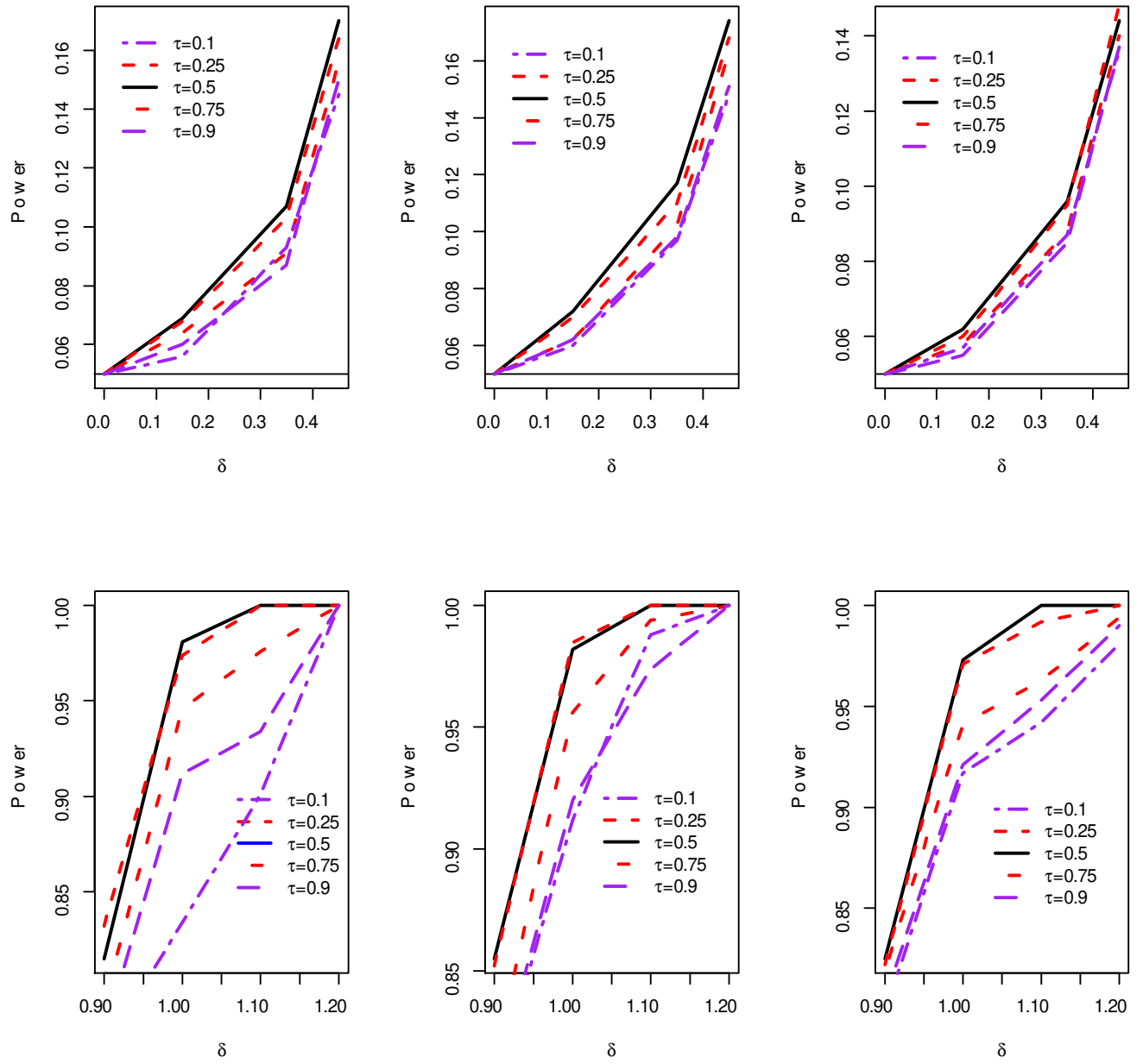
Figure 4 Magnified version of Figure 3 for 0 \leq \delta \leq 0.4 and 0.9 \leq \delta \leq 1.2 .
