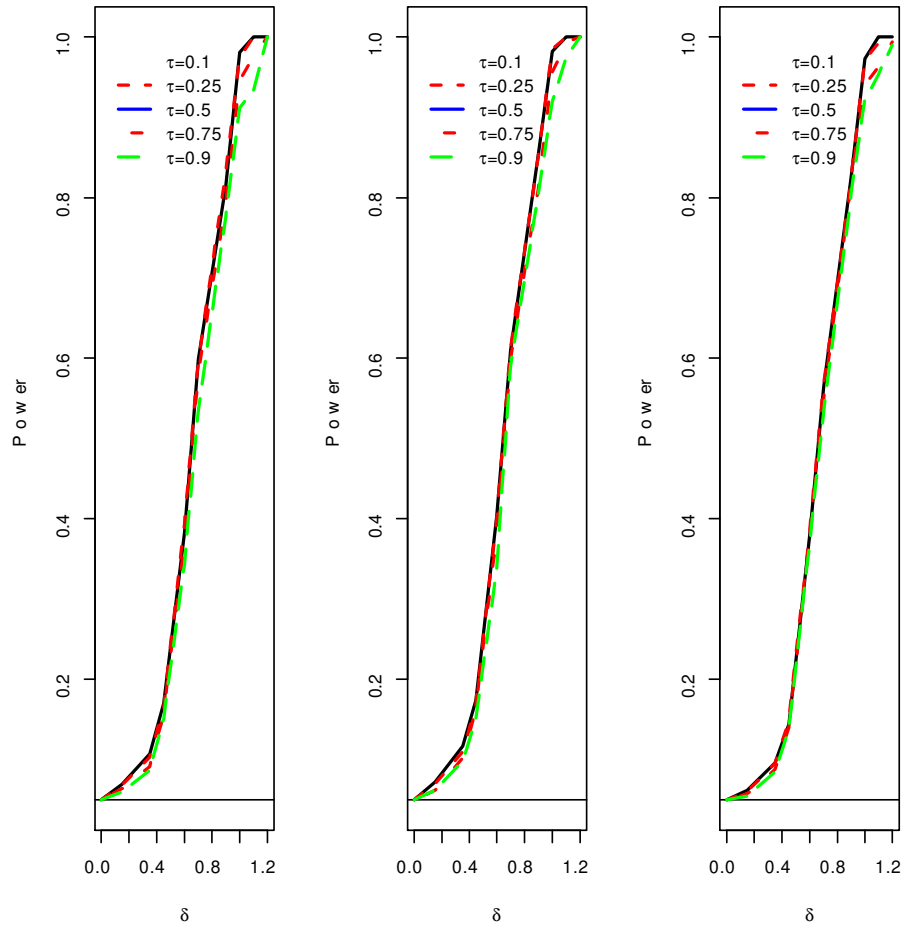
Figure 3. Finite sample power for the test statistic \max_j W_l(x_{2j}^*) for (5.5) with \chi^2(4) errors and n = 100 . Left panel Kaplan-Meier estimator, centre panel Breslow's (1972) estimator and right panel local Kaplan-Meier estimator of the unknown survival distribution G_0 .
