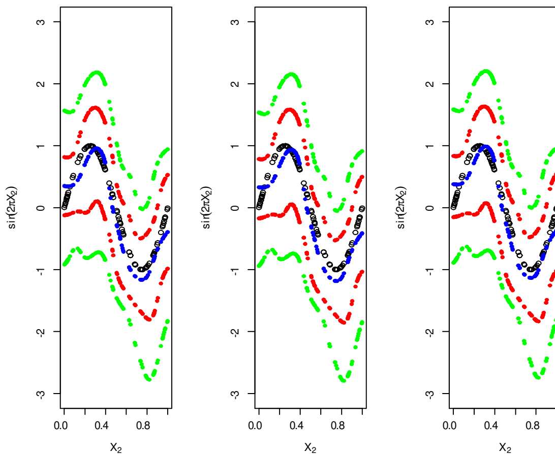
Figure 1. Quantile estimates (full circles) for \tau = (0.10, 0.25, 0.50, 0.75, 0.90) of the unknown nonparametric component \theta_{0\tau}(X_{2i}) = \sin(2\pi X_{2i}) (empty circle). Left panel Kaplan-Meier estimator, centre panel Breslow's (1972) estimator and right panel local Kaplan-Meier estimator of the unknown survival distribution G_0 .
