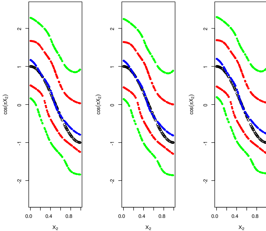
Figure 2. Quantile estimates (full circles) for \tau = (0.10, 0.25, 0.50, 0.75, 0.90) of the unknown nonparametric component \theta_{0\tau}(X_{2i}) = \cos(\pi X_{2i}) (empty circle). Left panel Kaplan-Meier estimator, centre panel Breslow's (1972) estimator and right panel local Kaplan-Meier estimator of the unknown survival distribution G_0 .
