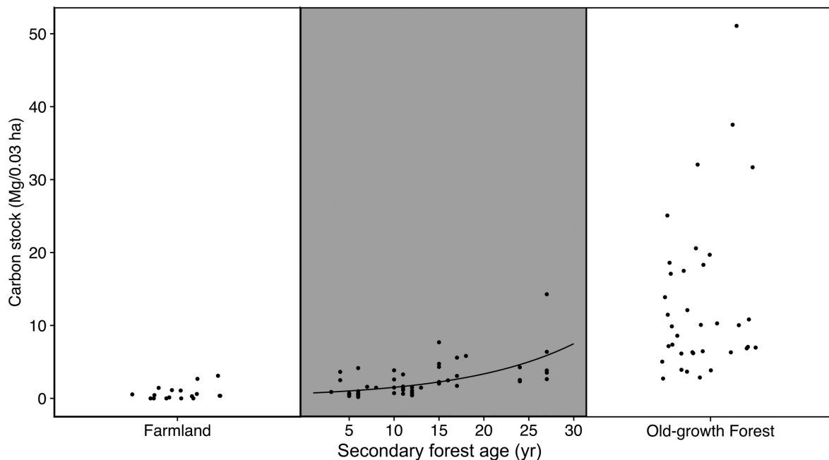
FIG. 2. Plots showing total carbon accumulation across the three habitats, farmland, secondary forest with age, and old-growth forest plots in Nagaland, northeast India. Black line in secondary forest (age in years) shows fitted linear mixed-effect model.
