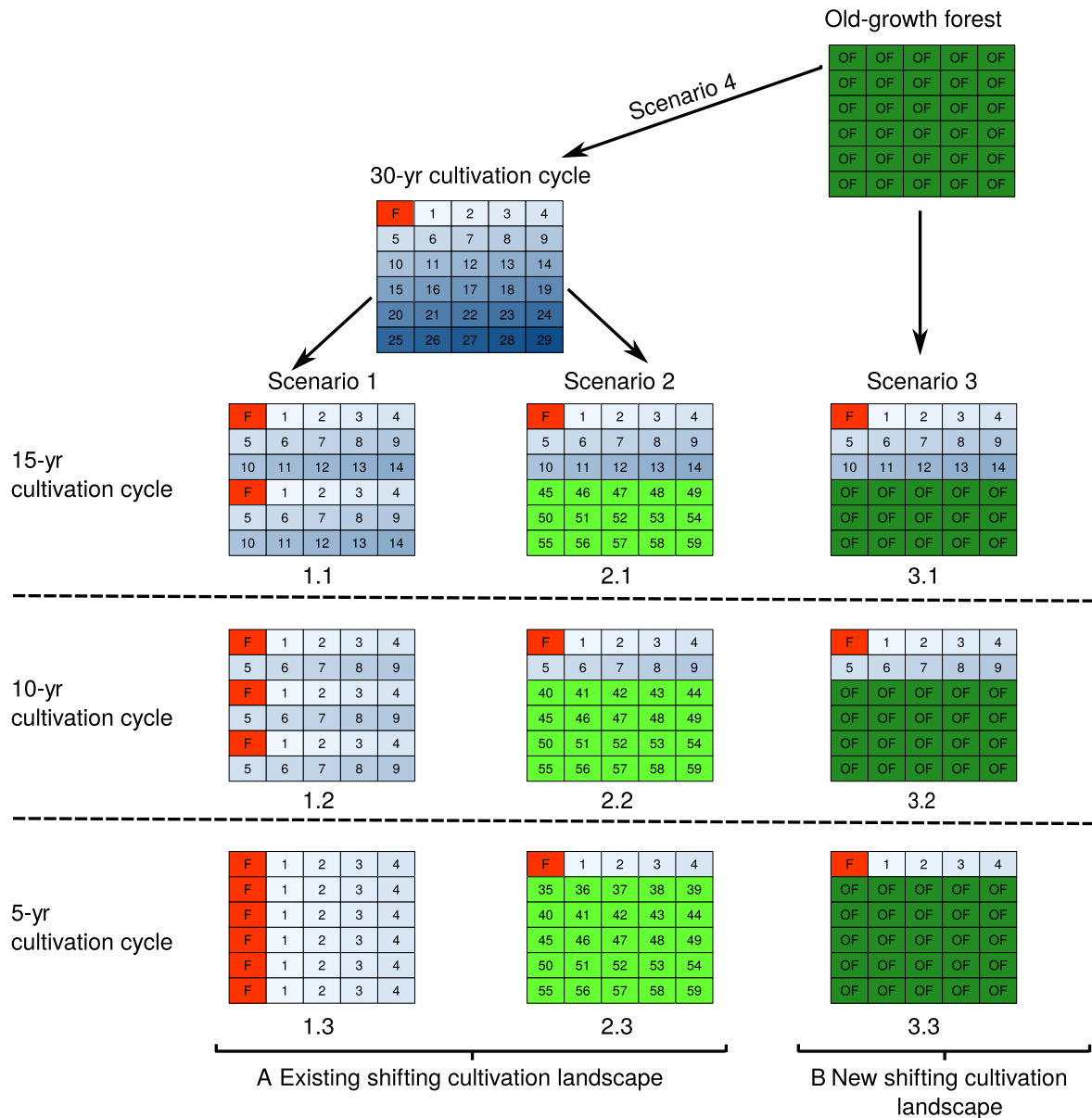
FIG. 1. The four sets of management scenarios used to predict changes in landscape carbon in (A) no forest sparing (Scenario 1) and secondary forest creation and sparing (Scenario 2) and (B) new shifting cultivation landscape with old-growth forest sparing (Scenario 3) and shifting cultivation expansion (Scenario 4). Colors indicate habitat types: farmland (F, red), active fallows (1–29 yr, different shades of blue), abandoned old fallows (>30 yr, light green), and old-growth forests (OF, dark green). Numbers within cells denote the age of the secondary forests; numbers under cell arrays indicate unique id for each landscape in a scenario.
