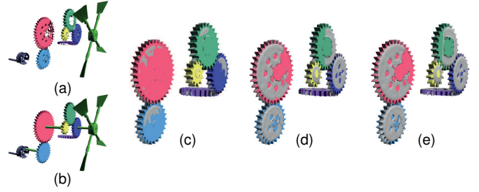
Fig. 10. (a) The scan of mechanical parts. (b) The final parametric model for these mechanical parts. (c-e) The comparison between scan and parametric parts obtained by local estimation, global optimization and local refinement respectively.
