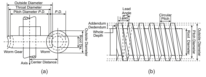
Fig. 17. Illustration of the nomenclature for worm and worm gear. (a) Two mating worm gear and worm. (b) Worm.
