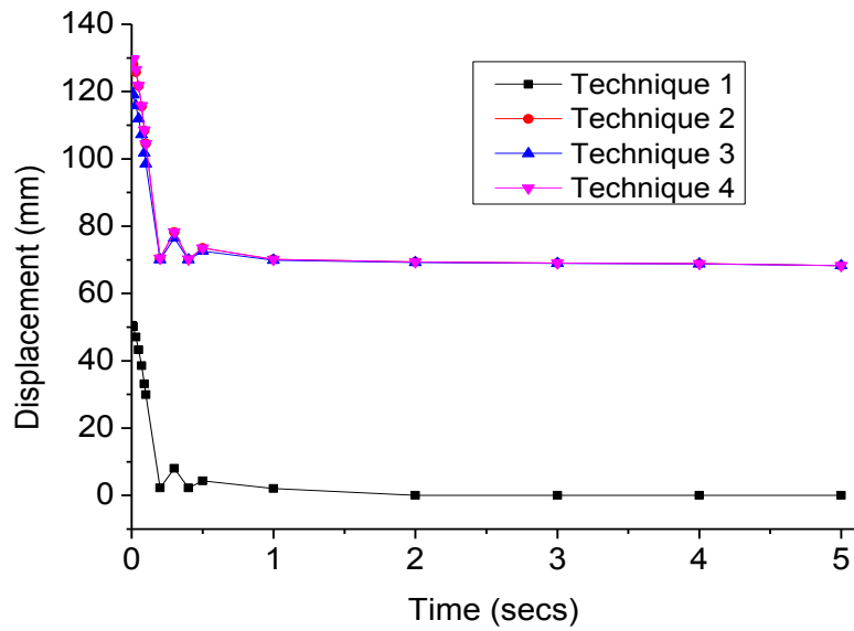
a) Displacement vs time (ECRS)
