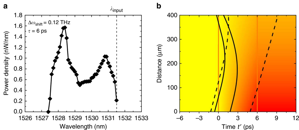
Fig. 5 Simulation of the FC front interaction with CW probe wave packets via ray tracing. a Wave packets average power spectrum for 6 \mu W average power of the CW probe at 1531.5 nm, rising time of the front of 6 ps, and initial band shift \Delta\omega_{\text{shift}} of 0.12 THz. Other parameters are listed in the Supplementary Note 6. b The trajectories of the probe wave packets with respect to the front velocity. The two vertical orange lines represent the extent of the index front with a rise time of 6 ps, while the shading represents the refractive index front as it exponentially decays during propagation inside the waveguide. Solid black lines represent those wave packets that undergo complete transitions, while the dashed lines depict the wave packets which only undergo incomplete transitions
